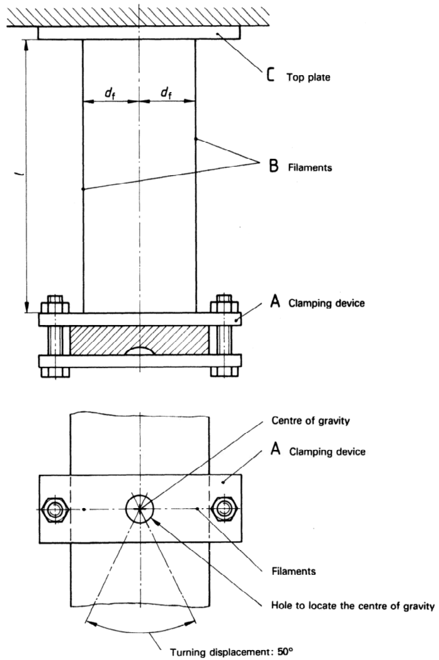
Figure – Measurement device for the determination of the polar moment of inertia
