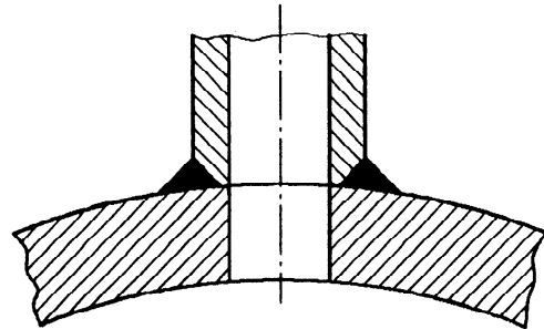
Figure 6 — Butt-welding for auxiliary connections
