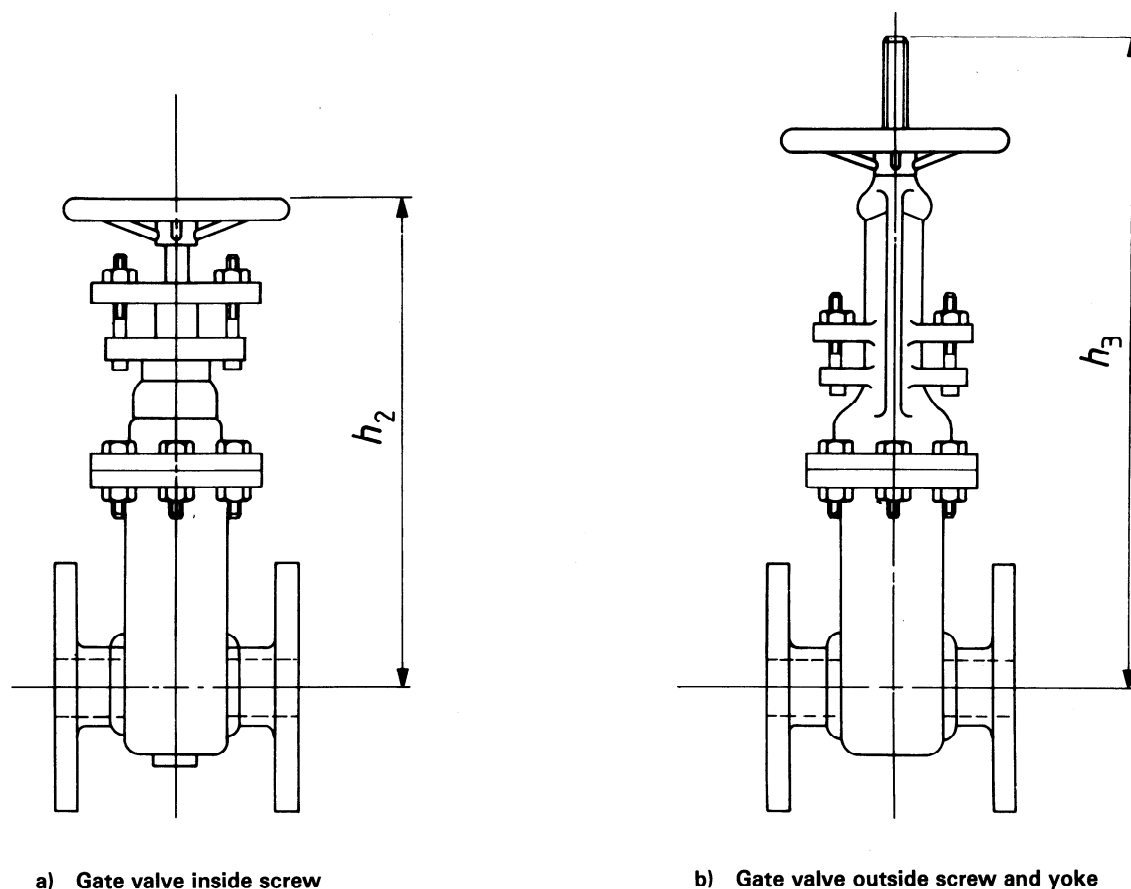
a) Gate valve inside screw
