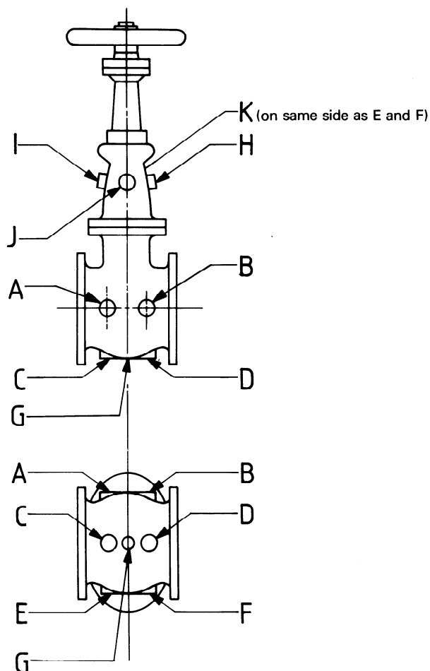
Figure 3 — Location of tappings for auxiliary connections
