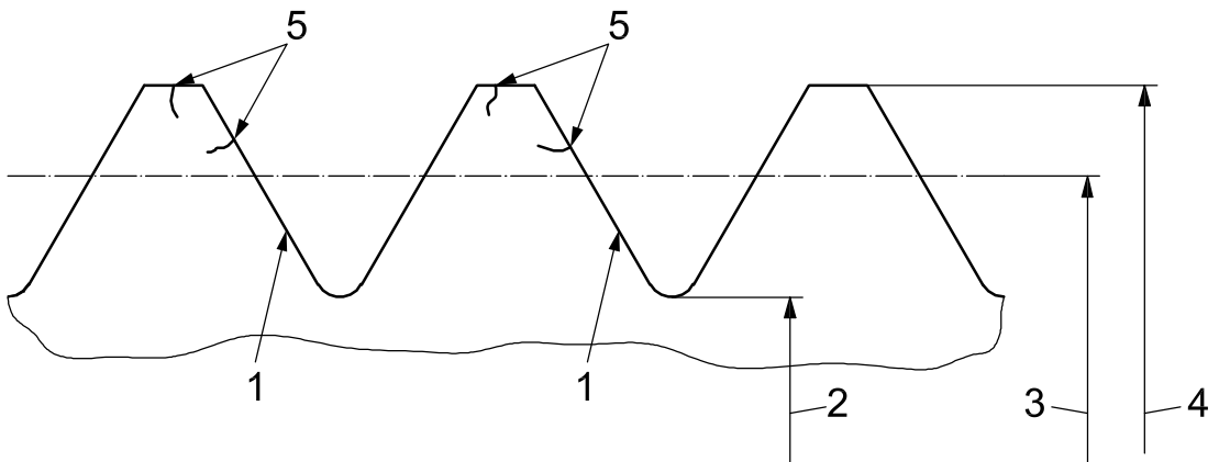
Figure 5 — Non-permissible laps, seams and surface irregularities in threads
