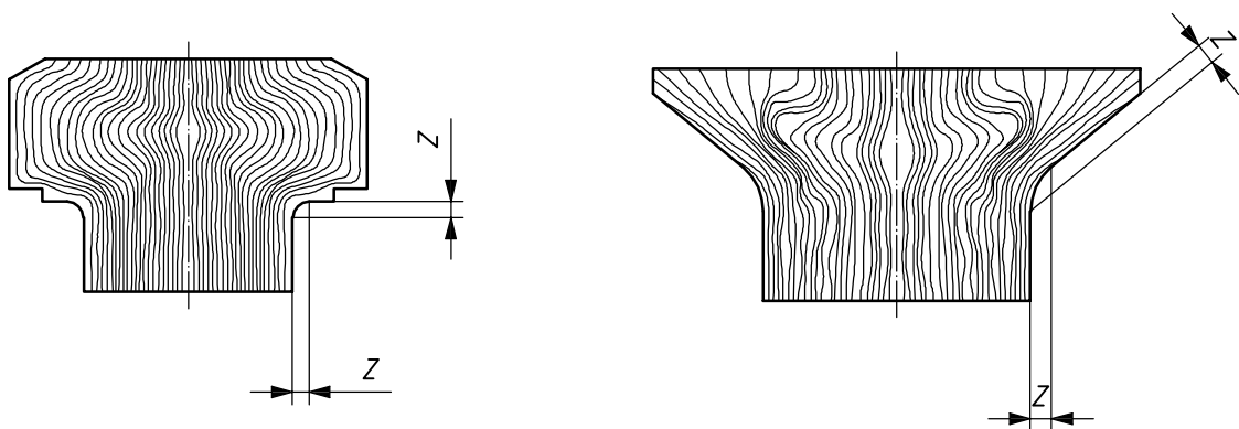
Figure 1 — Distortion in head-to-shank fillet area (see 5.3.5)
