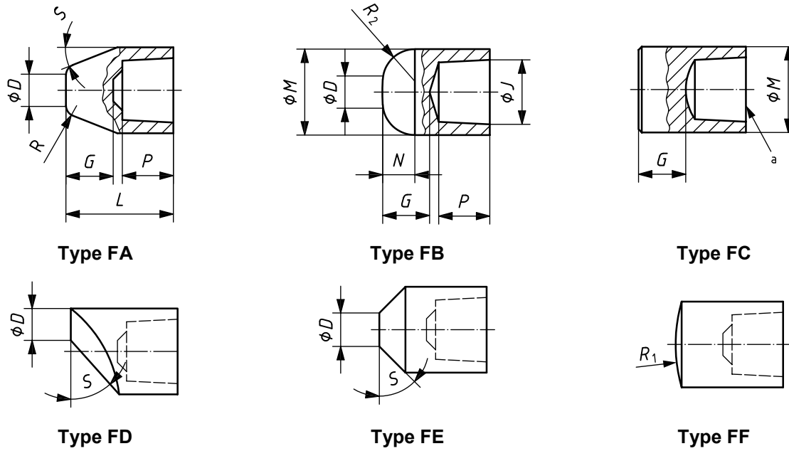
Figure A.1 — Alternative female electrode caps
