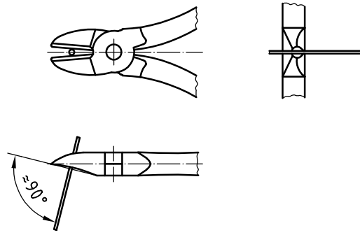
Figure 8 — Diagonal cutting nippers
