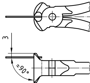
Figure 9 — End cutting nippers
