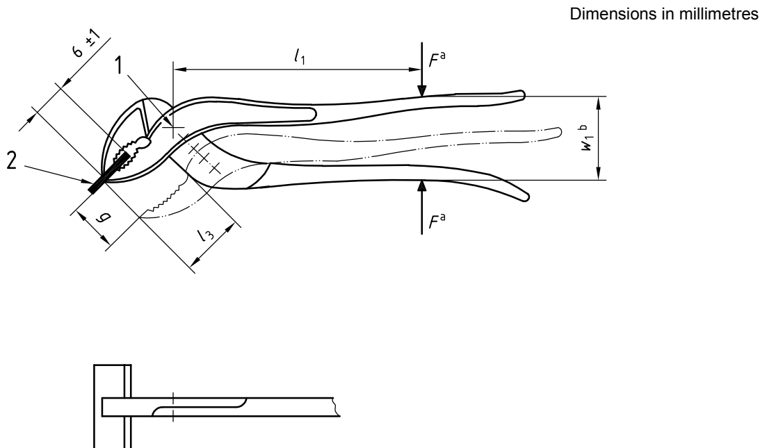
Figure 3 — End cutting nippers
