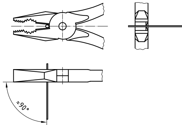
Figure 10 — Combined gripping and cutting pliers e.g. engineer's pliers or lineman's pliers
