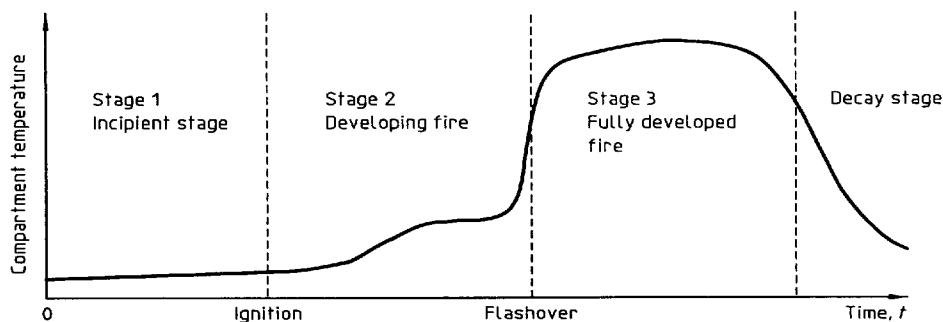
Figure 2 — Diagram showing the different phases in the development of a fire within a compartment
