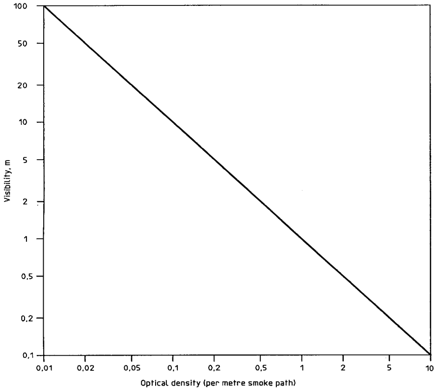
Figure 1 — Relationship between optical density and visibility (after Jin 1978 [5] — see annex B)
