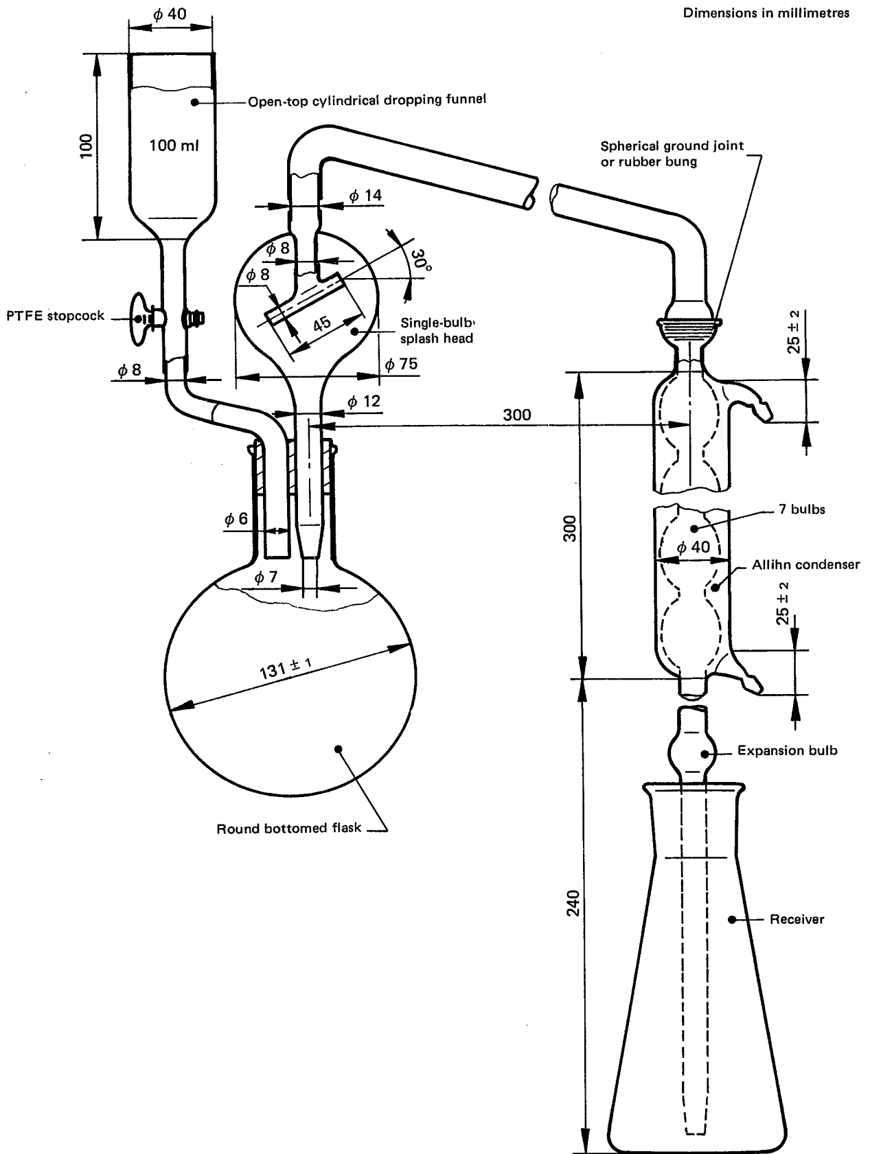
Figure — Typical distillation apparatus
