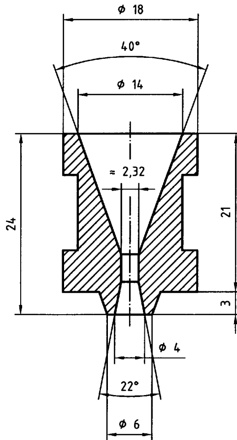
Figure A.3 — Bottom orifice
