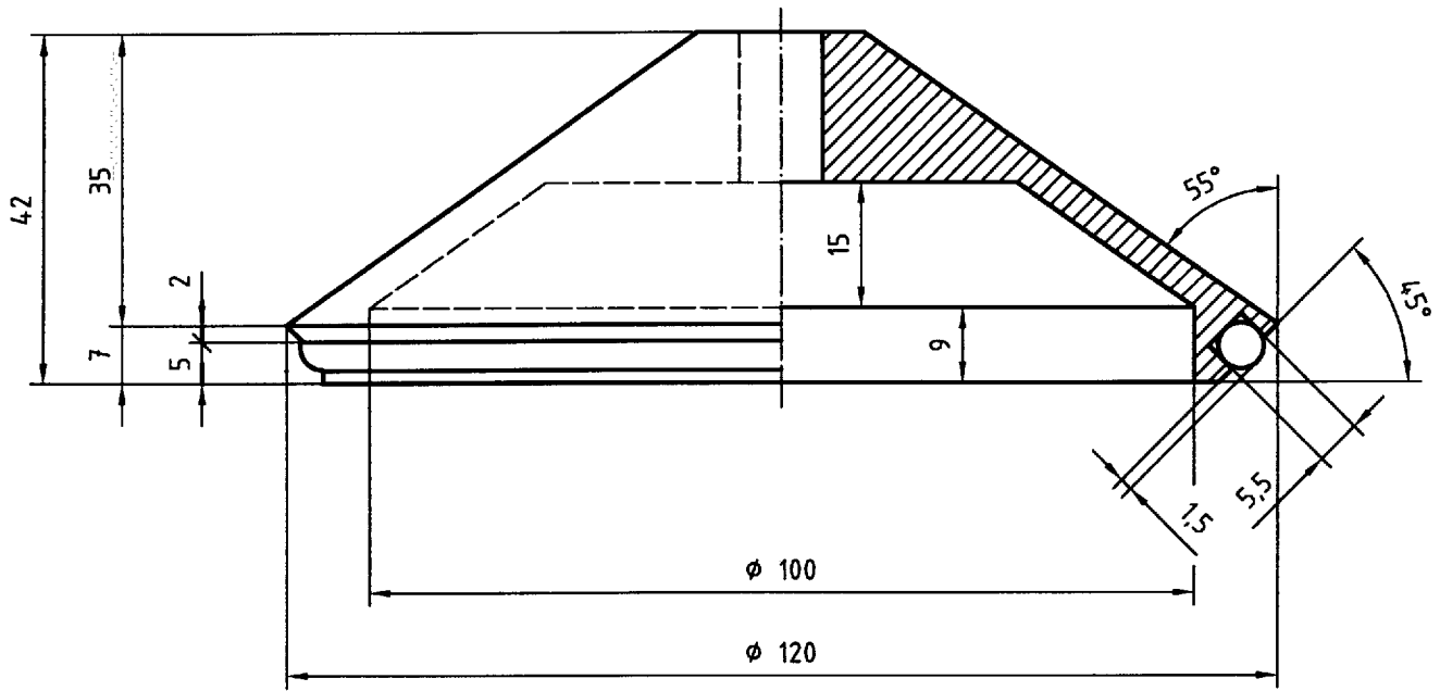
Figure A.2 — Sealing cone
