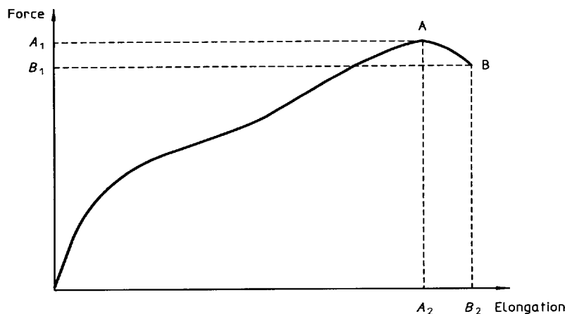
Figure 1 — Typical force/elongation curve
