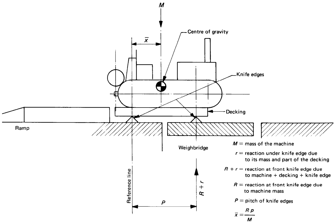
FIGURE 1 — Determination of the fore-and-aft co-ordinate, \bar{x}
