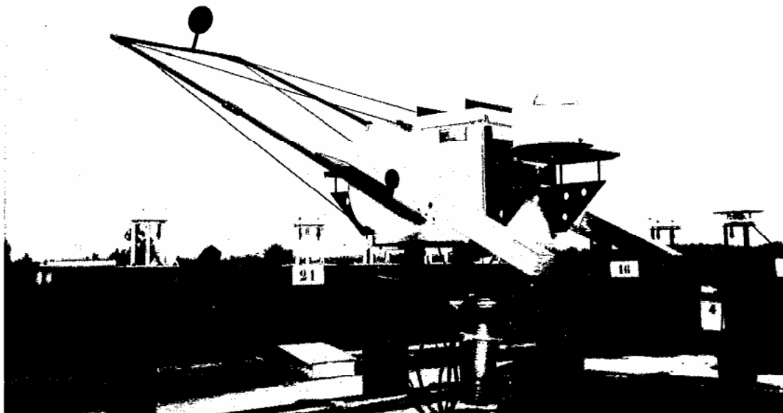
Figure 2 — Kipp and Zonen CM 10 ventilated pyranometer on a suntracker in the shade disc configuration, at the SETIM Observatory at Carpentras, France
