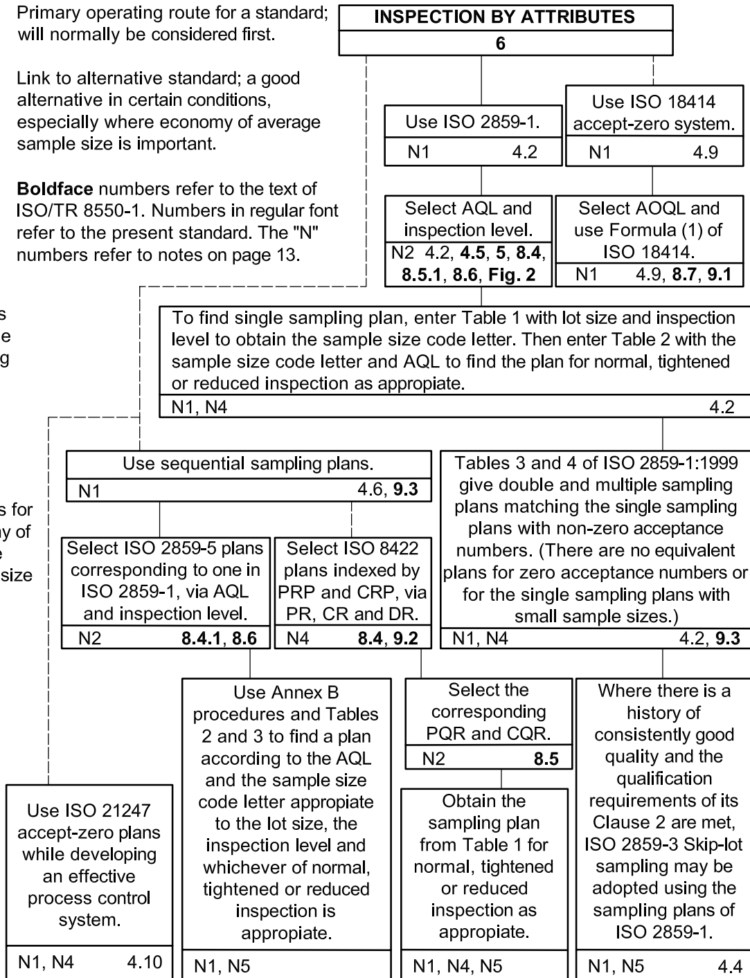
Figure 1 — Illustration of the selection procedure for inspection by attributes when production is continuous and run length exceeds 10 lots on original inspection
