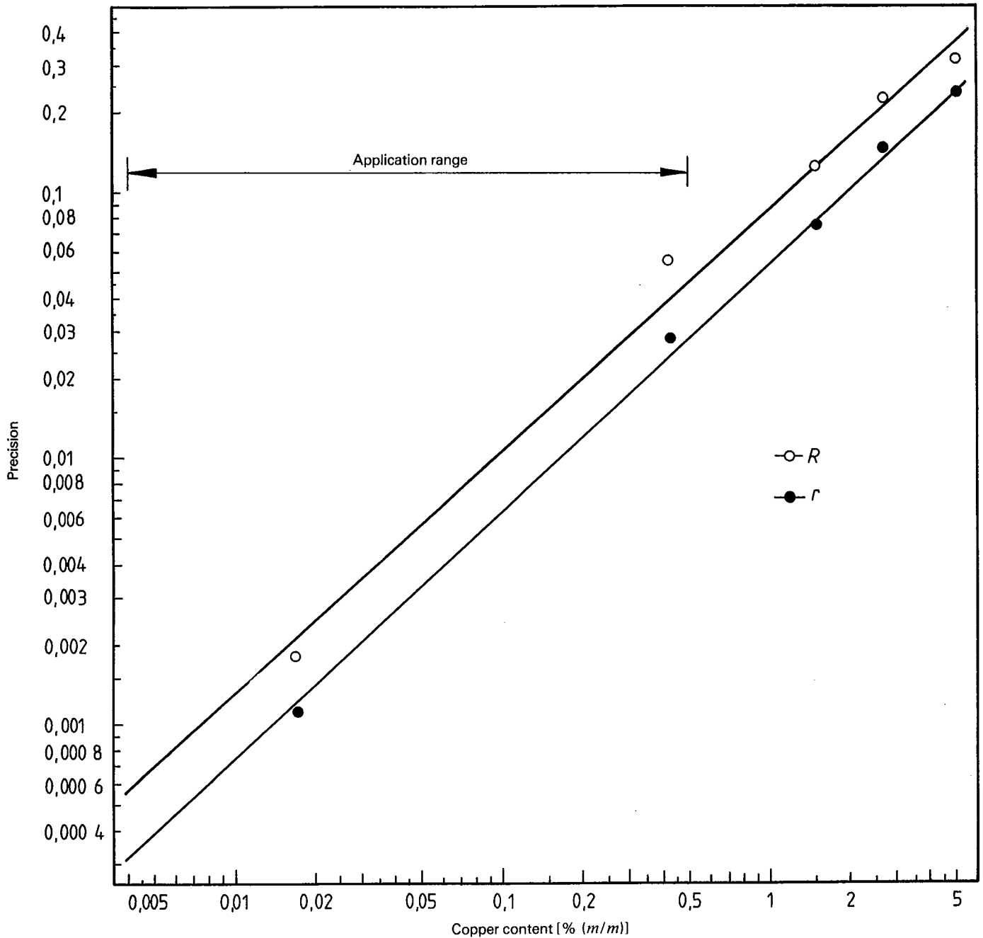
Figure — Relationship between copper content and repeatability, r , or reproducibility, R
