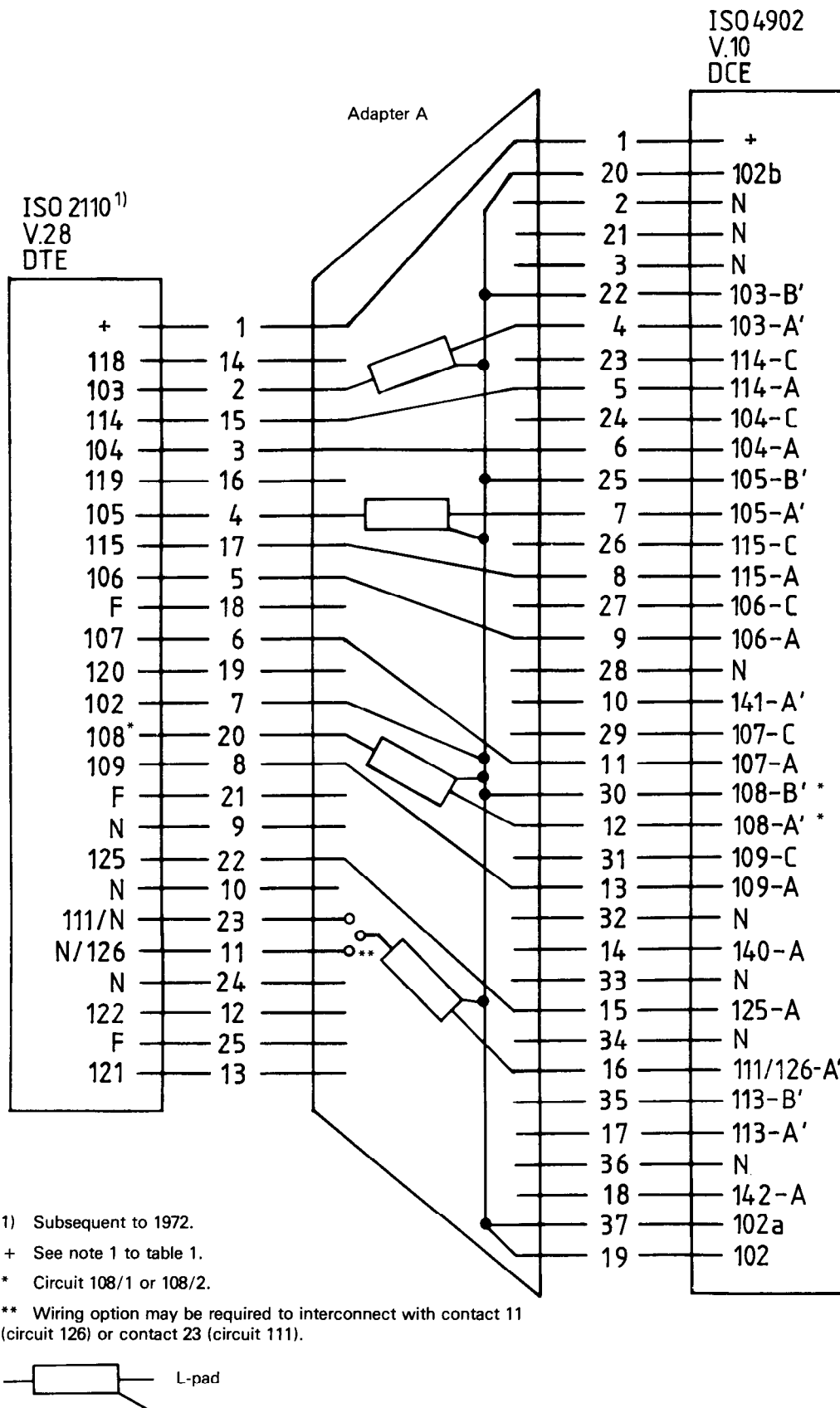
Figure C.5a) – 37/25-pole basic adapter, configuration A
