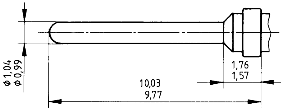
Figure 4 — Male contact
