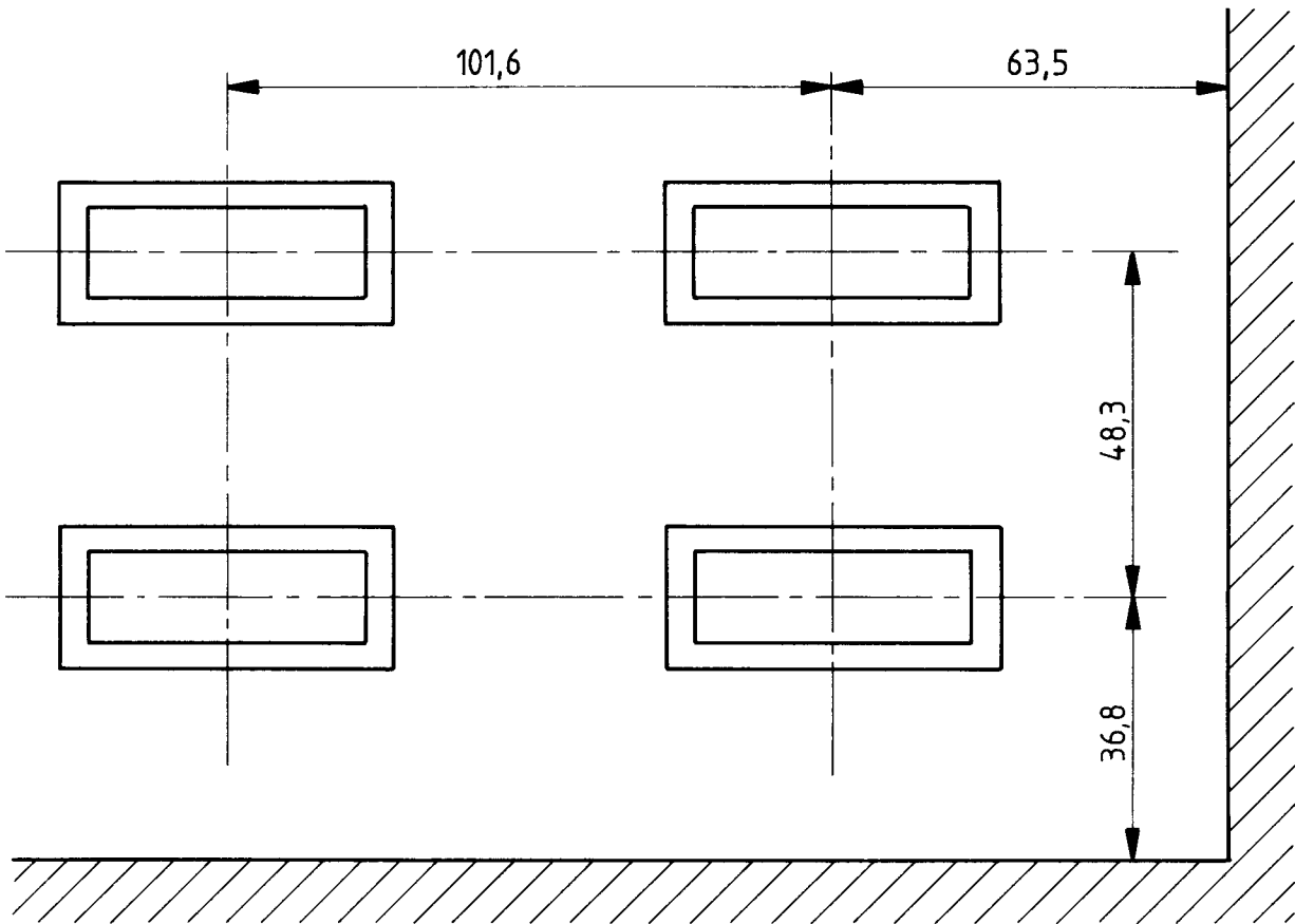
Figure A.2 – Minimum DCE connector spacing
