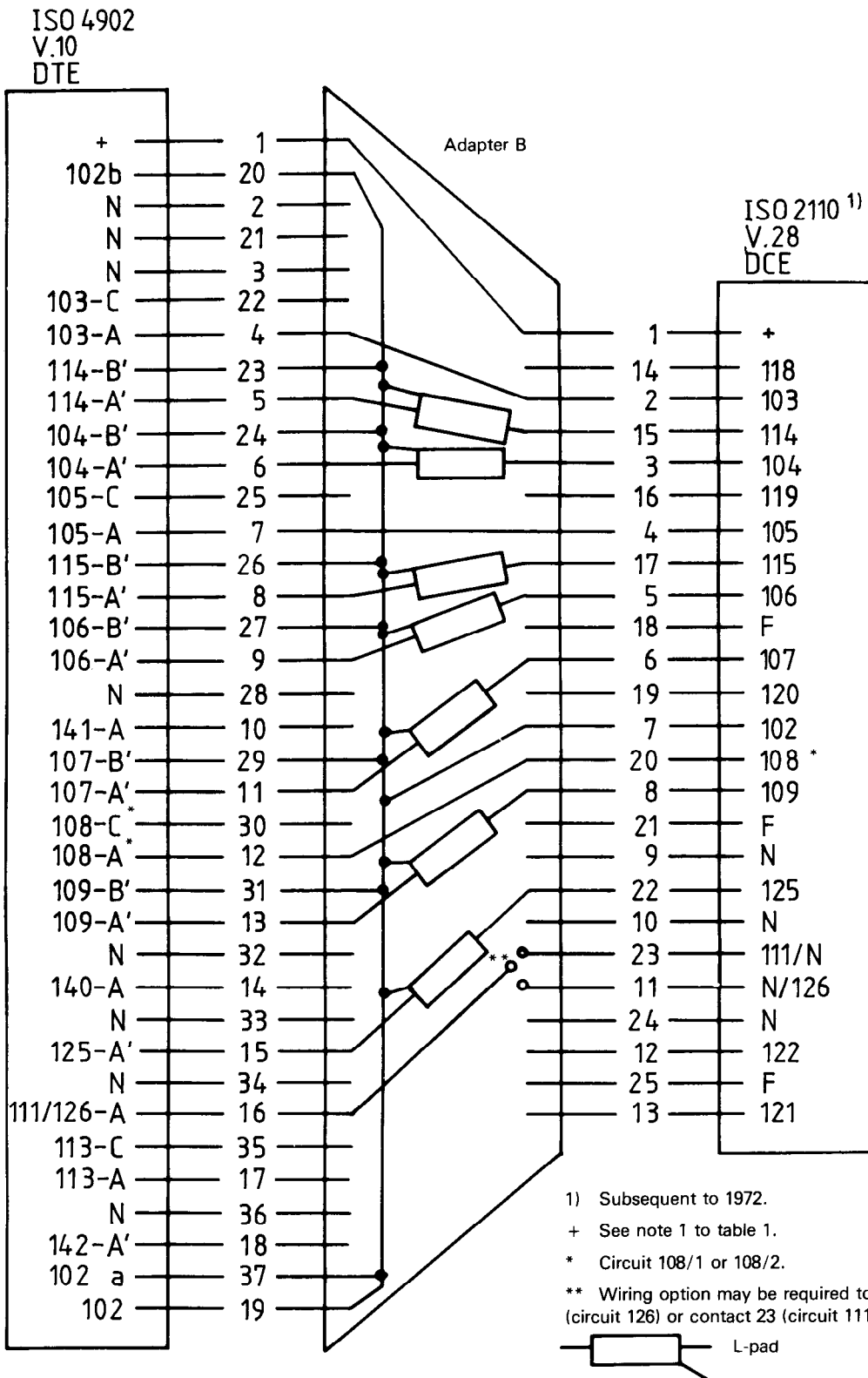
Figure C.5b) – 37/25-pole basic adapter, configuration B
