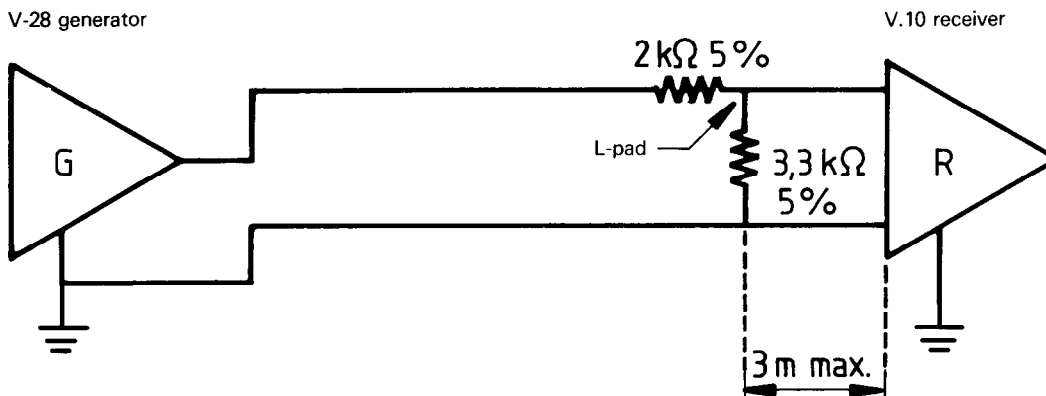
Figure C.3 – L-pad attenuator for protection of V.10 receiver
