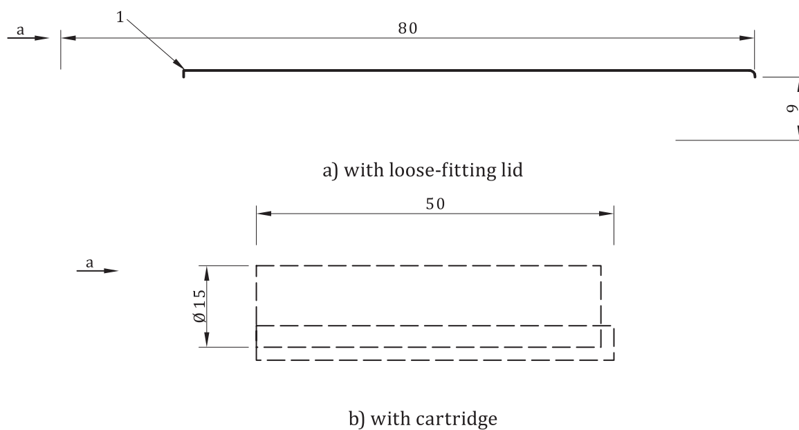
Figure 1 — Combustion apparatus
