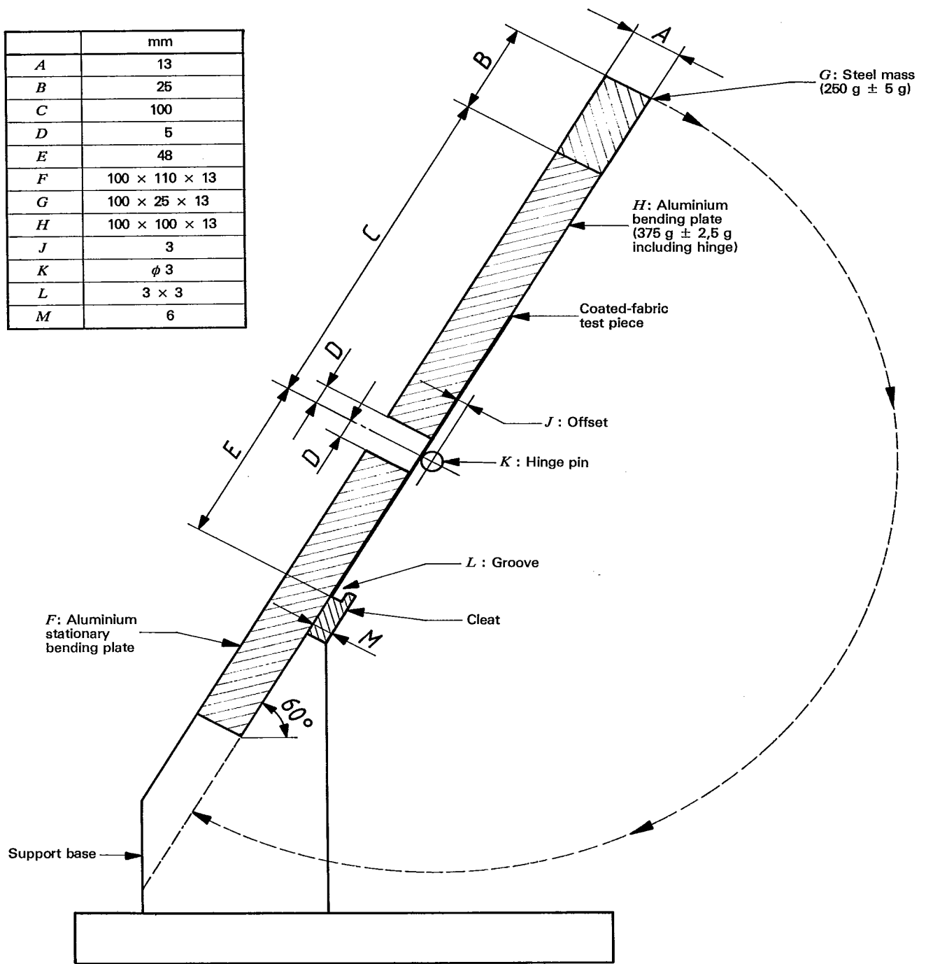
Figure 2 — Dimensions of bending jig
