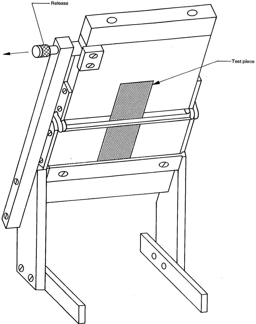
Figure 1 — Bending jig for coated fabrics
