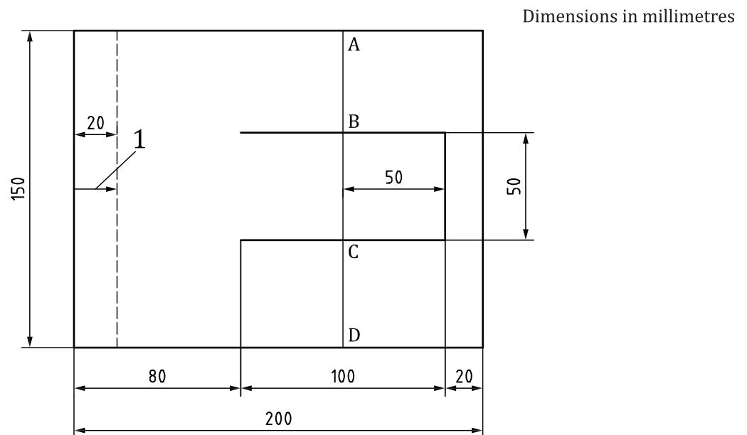
Figure 1 — Principle of tongued test piece
