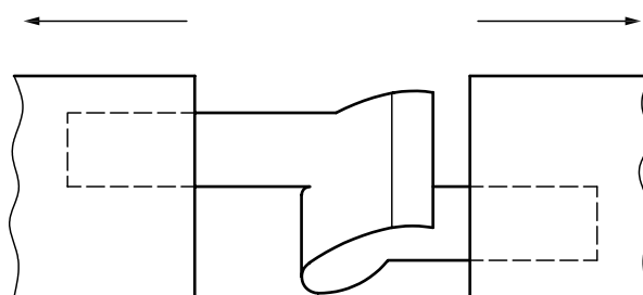
Figure 6 — Clamping of trouser-shaped test piece
