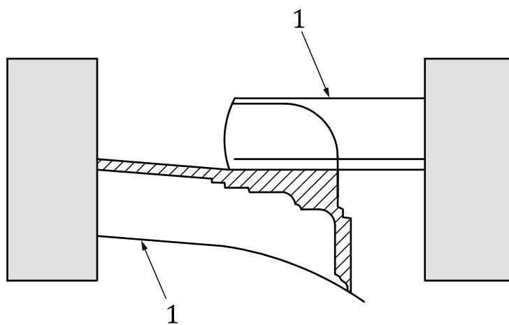
Figure B.1 — Wide-width trouser-shaped test piece
