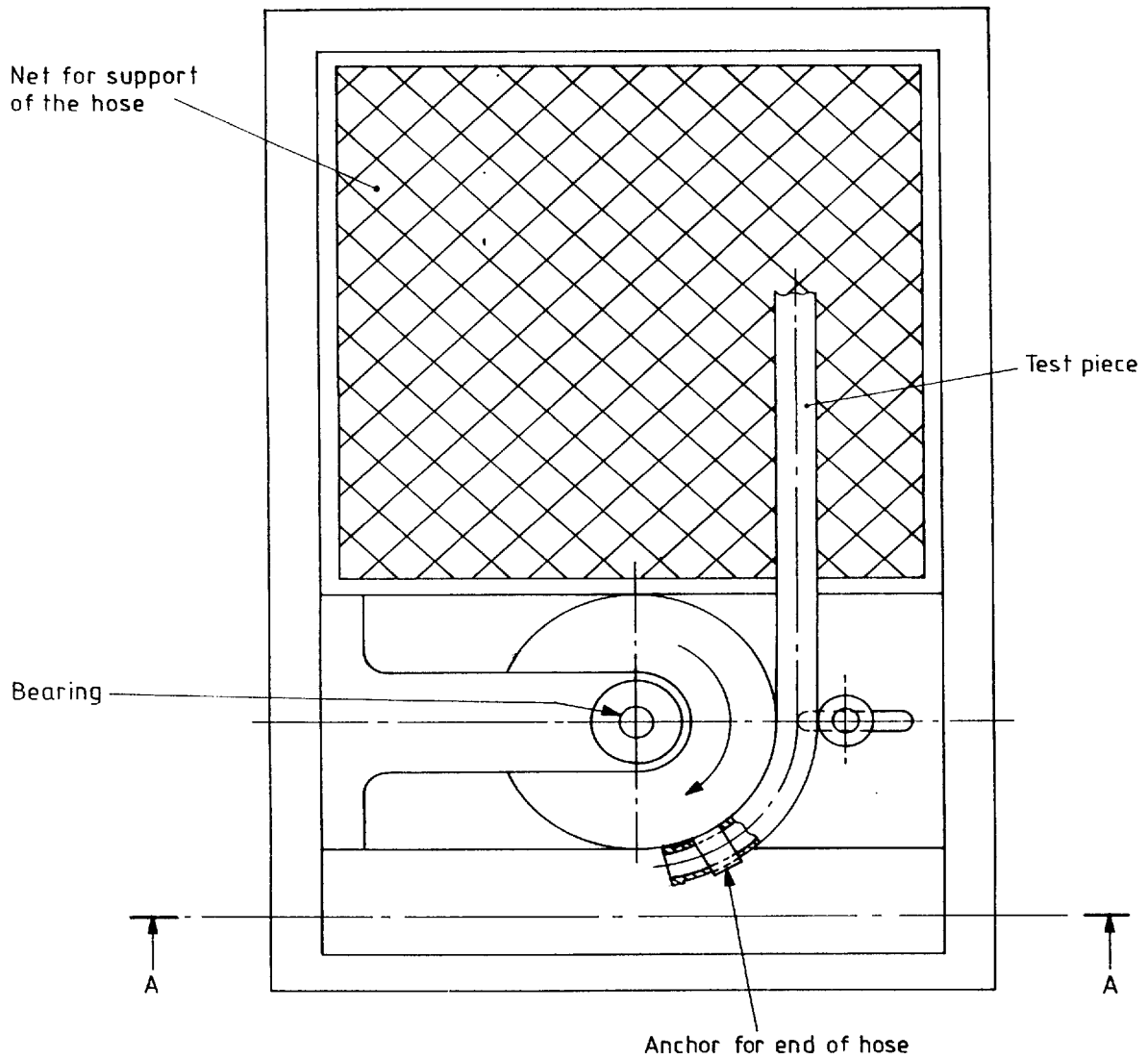
Figure 1 - Apparatus for method A
