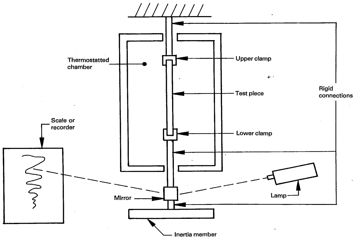
Figure 1 — Uncompensated free oscillation apparatus with inertia member suspended below the test piece
