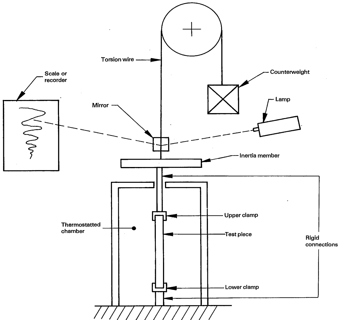
Figure 2 — Uncompensated free oscillation apparatus with counterweighted inertia member suspended above the test piece
