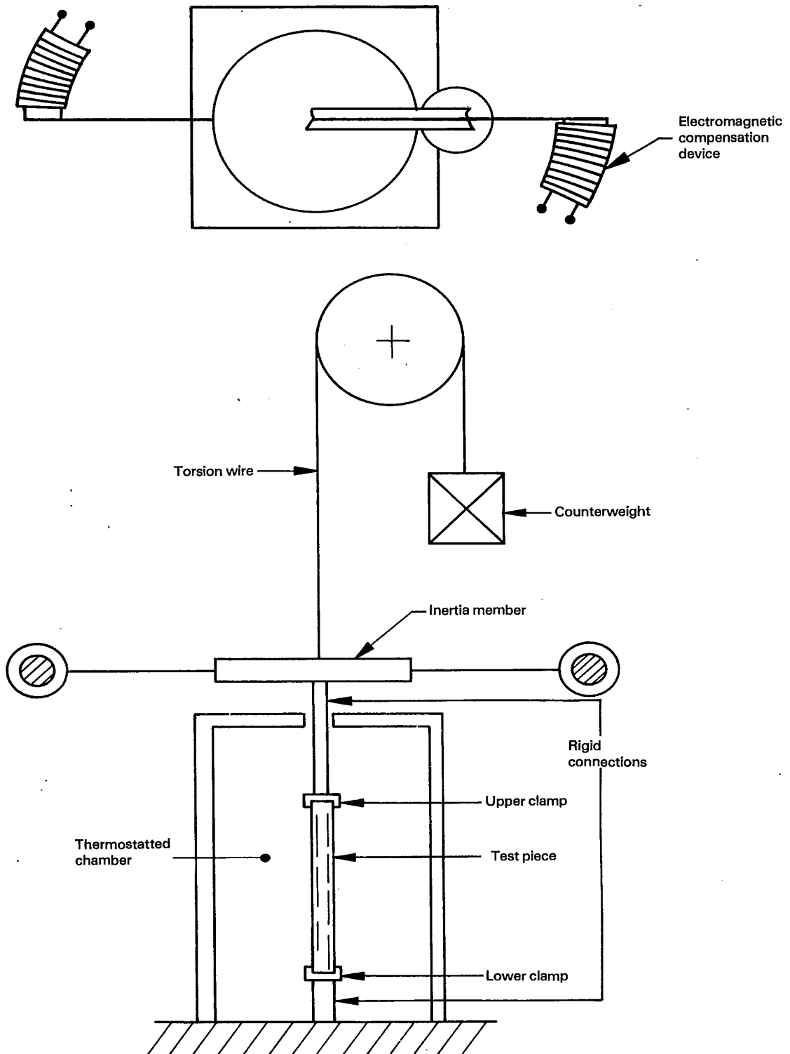
Figure 3 — Forced resonance oscillation device
