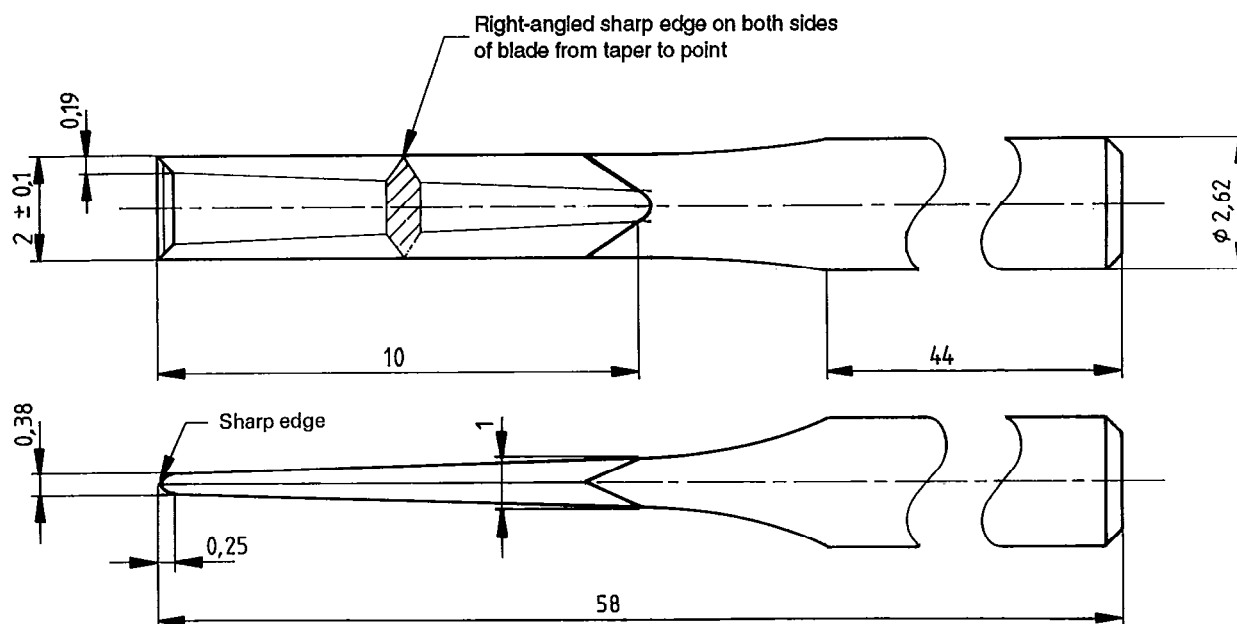
Figure C.2 — Piercing chisel
