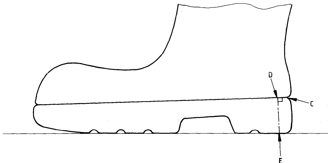
Figure A.1 — Measurement of heel thickness
