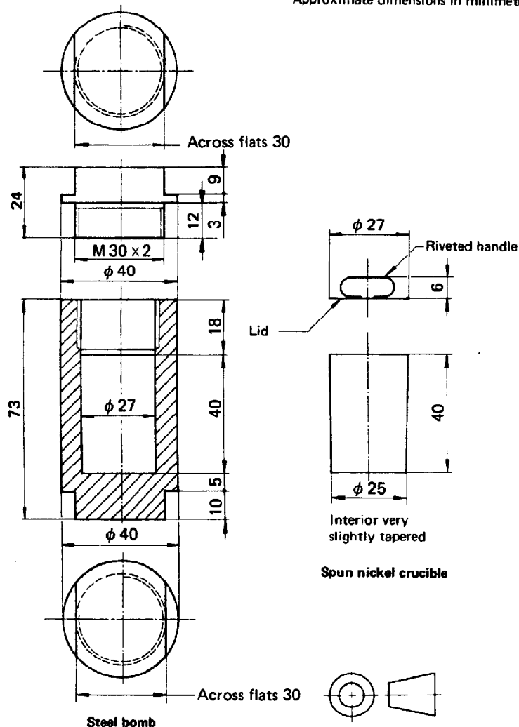
FIGURE 1 – Combustion bomb, gas-fired type (for method A)
