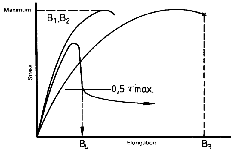
Figure 1 — Failure criteria for method B
