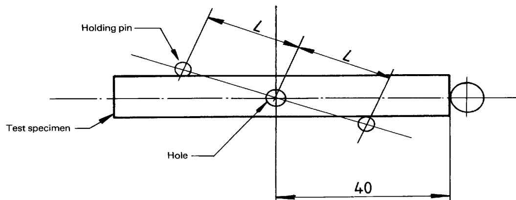
Figure 2 — Fixture for drilling holes in test specimens
