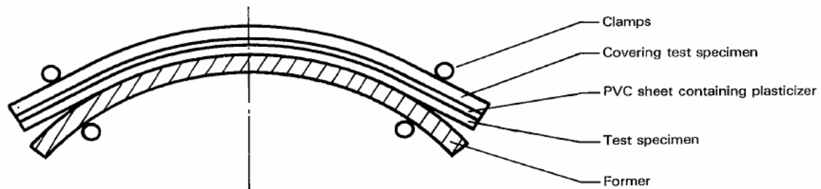
Figure 2 — Example of sandwiched test specimen
