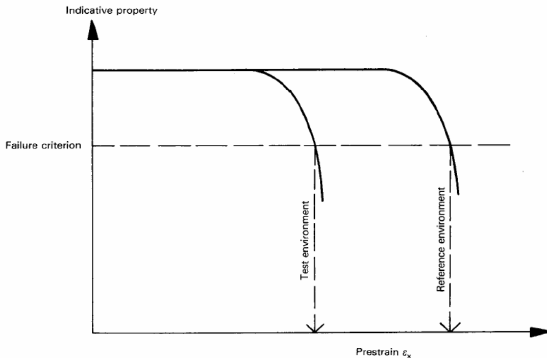
Figure 3 — Graphical evaluation of test results
