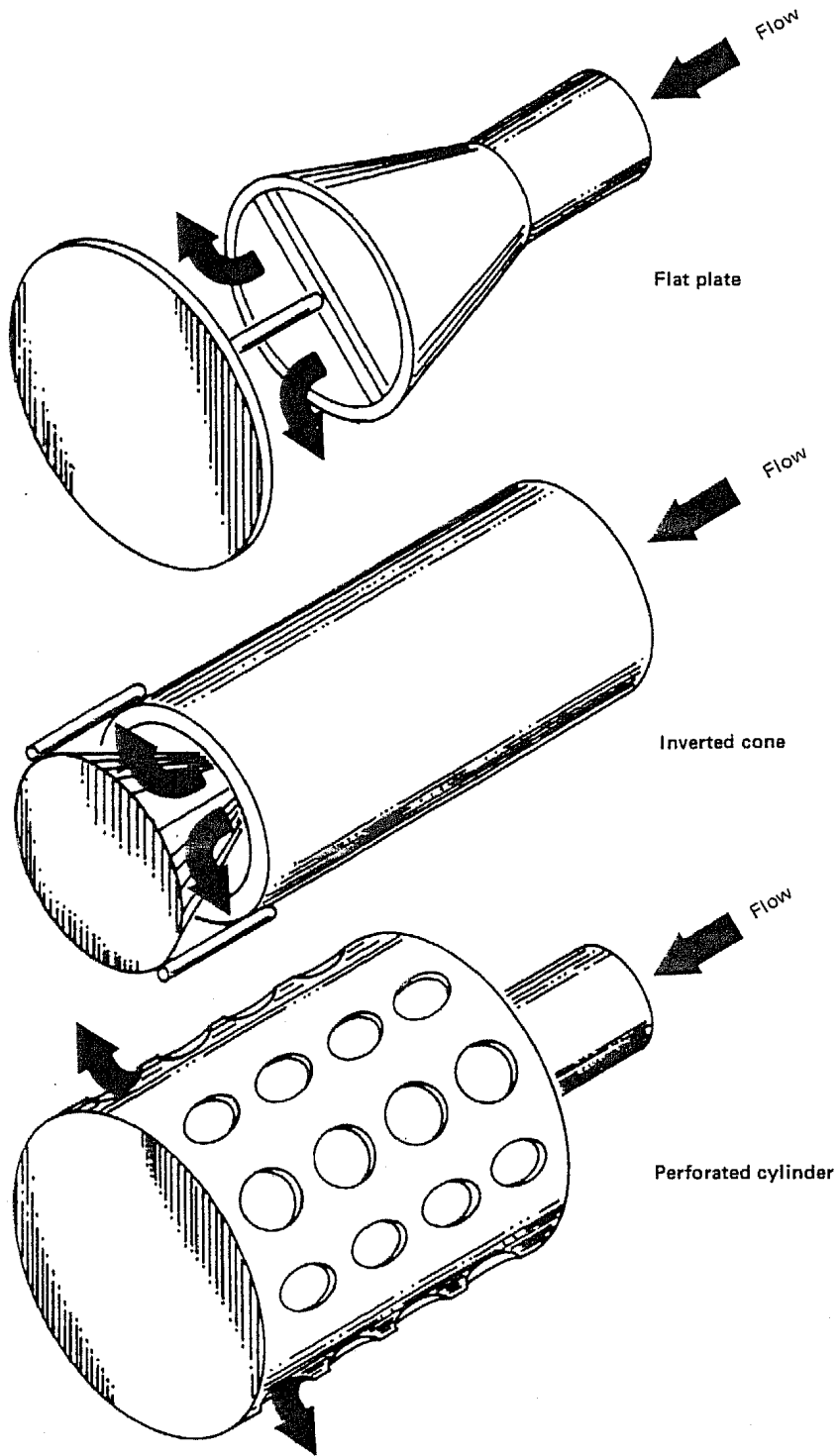
Figure 8 — Typical diffuser designs
