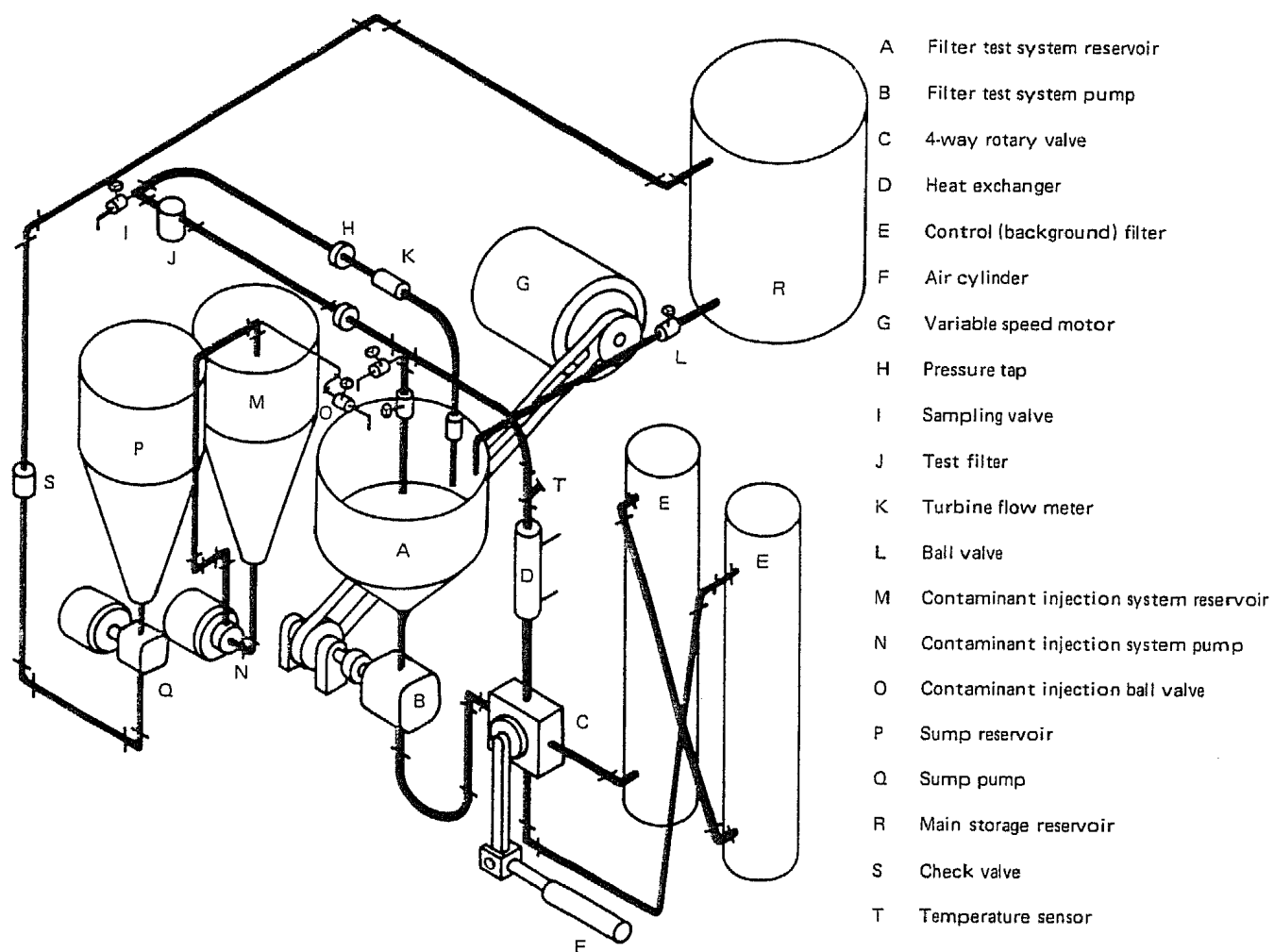
Figure 2 — A typical filter performance test system
