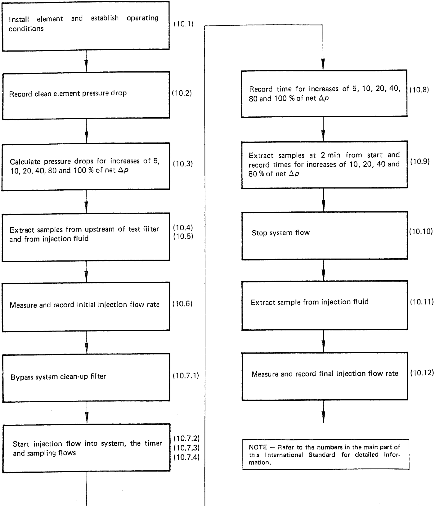
Figure 6 — Procedural diagram for filter performance test
