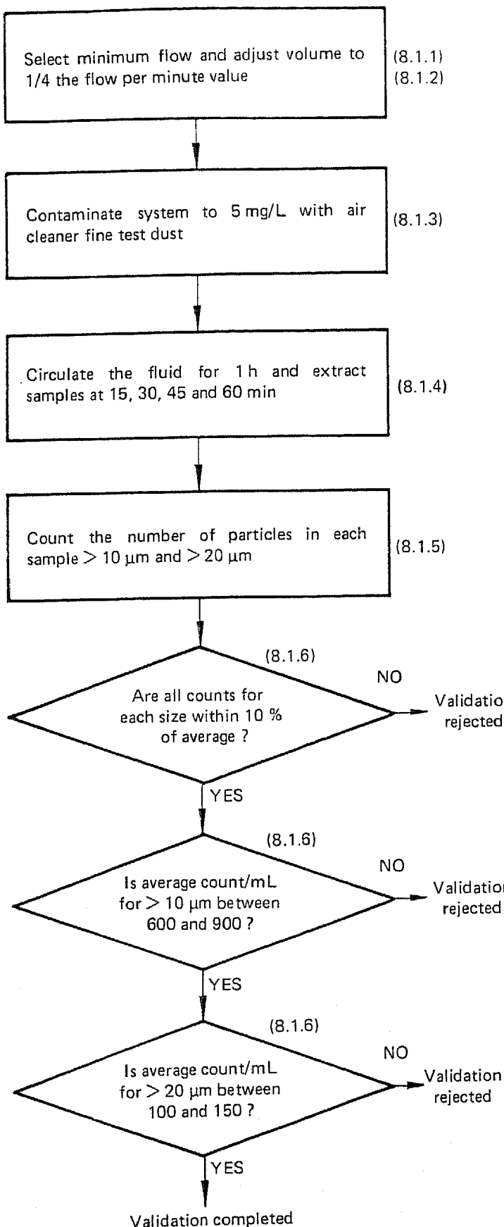
Figure 4 — Procedural diagram for validation
