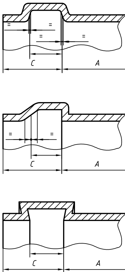
Figure 3 — Typical groove designs for elastomeric ring seal sockets
