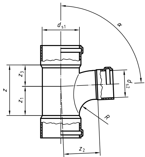
Figure 16 — Reducing branch with only sockets (swept)
