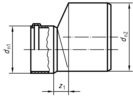
Figure 12 — Reducer
