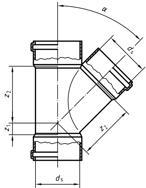
Figure 14 — Branch with only sockets (unswept)
