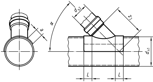
Figure 17 — Saddle branch
