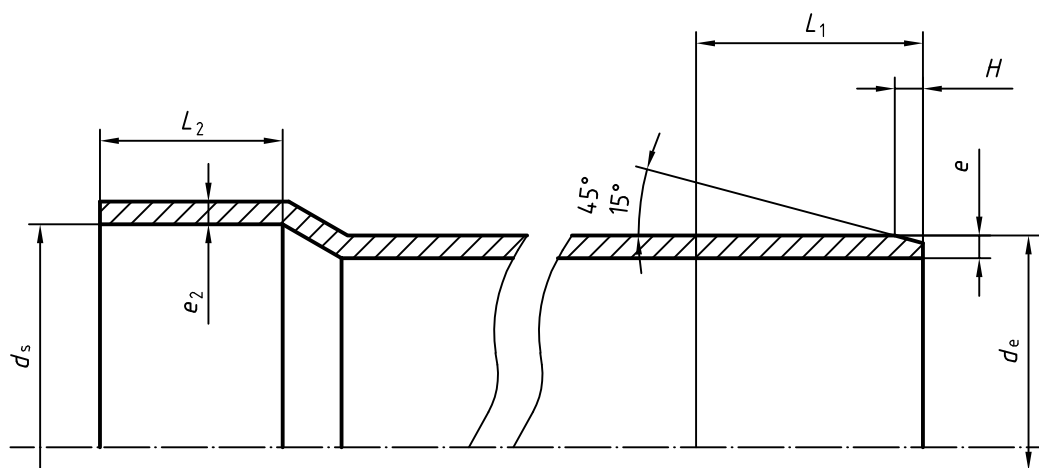
Figure 6 — Basic dimensions of sockets and spigots for solvent cement joints
