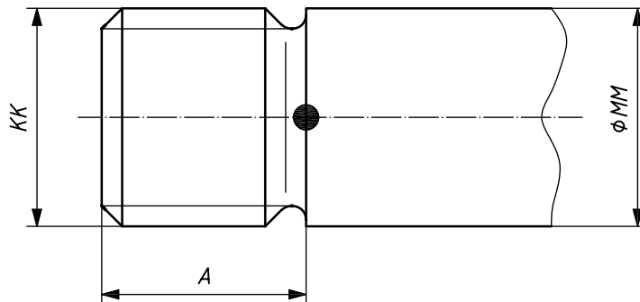
Figure 8 — Male thread without shoulder for pneumatic cylinder piston rods
