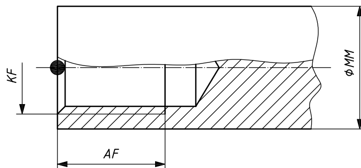
Figure 9 — Female thread for pneumatic cylinder piston rods
