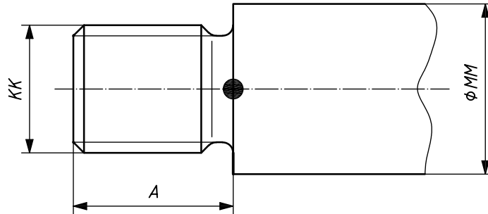
Figure 7 — Male thread with shoulder for pneumatic cylinder piston rods
