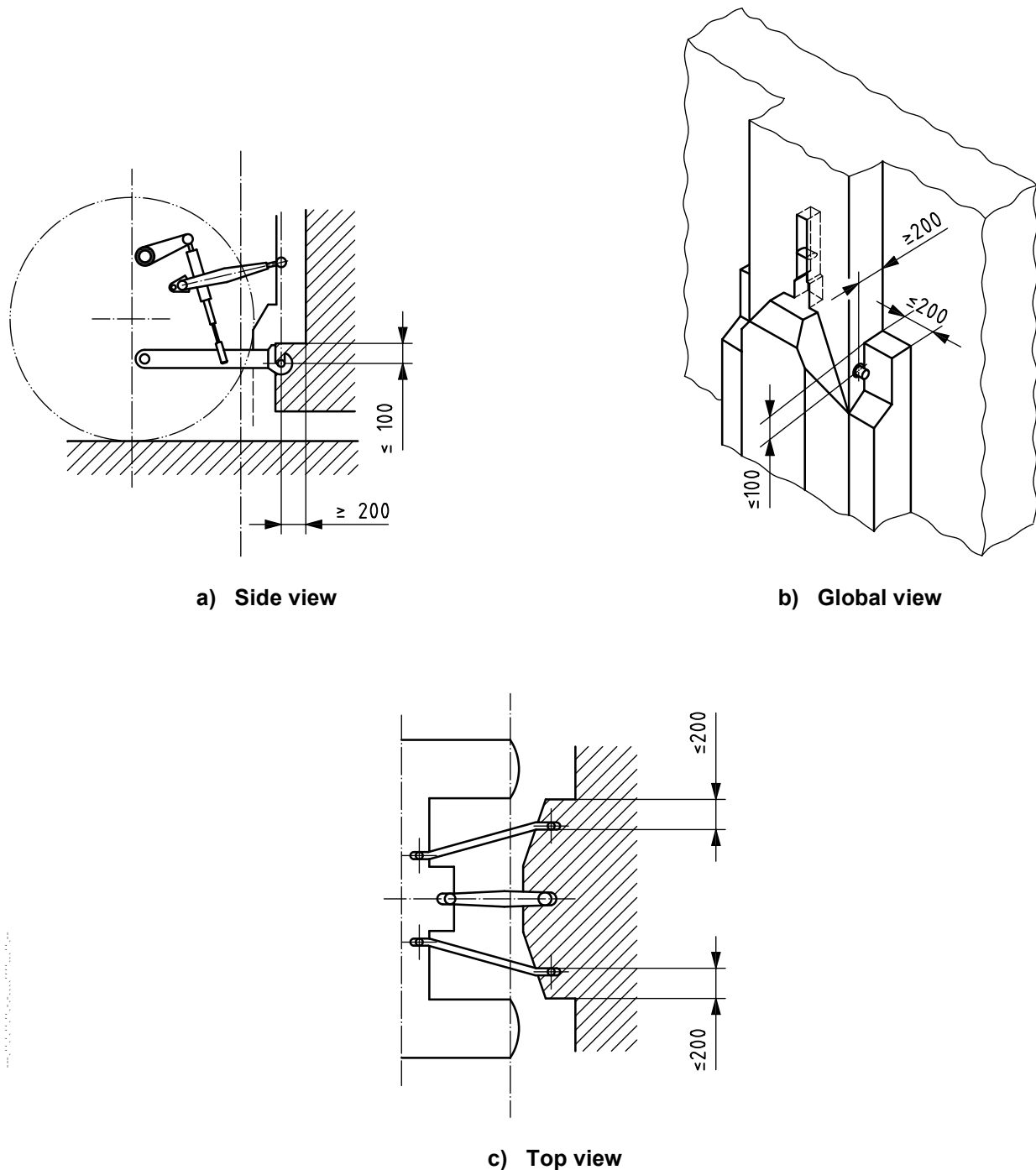
Figure 5 — Clearance zone
