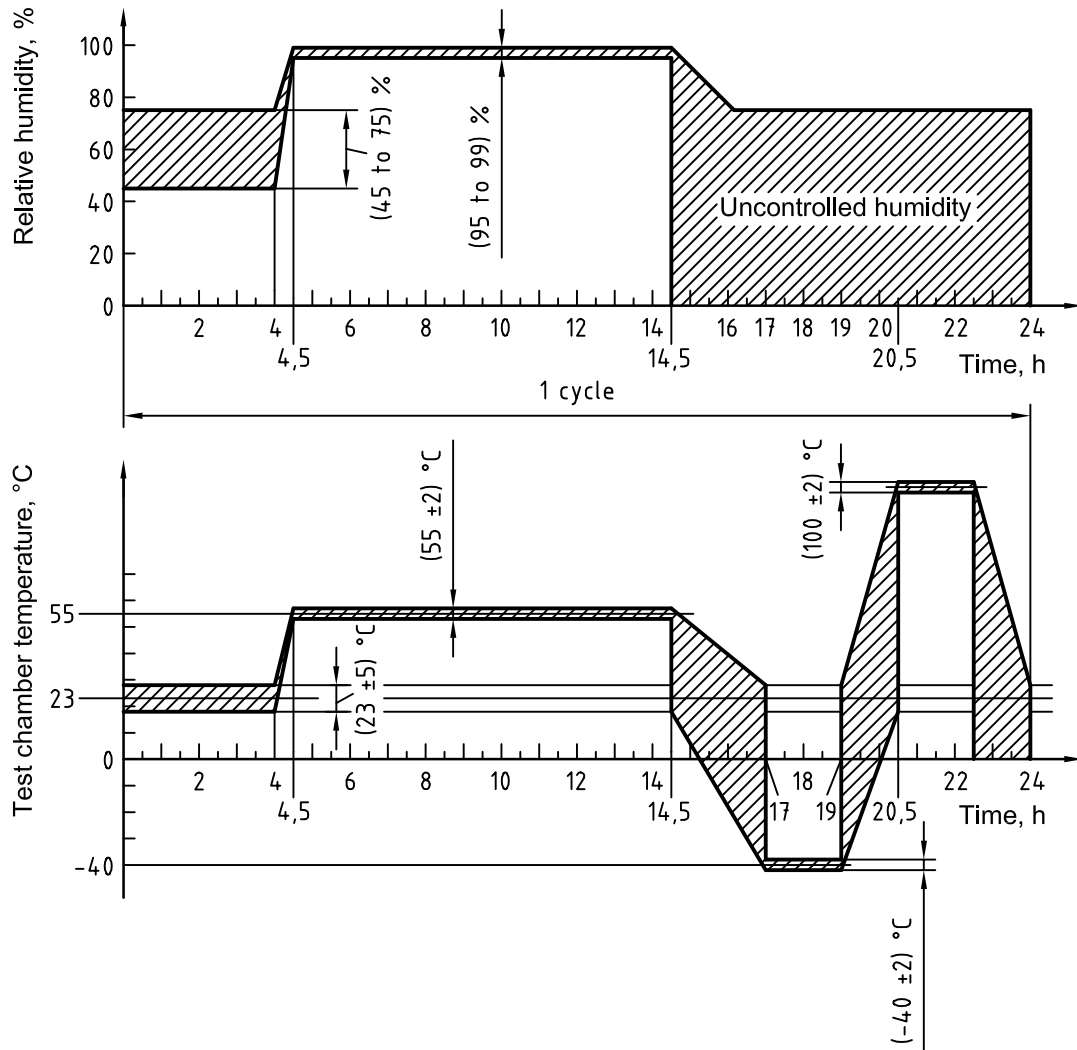
Figure 11 — Temperature/humidity cycling test
