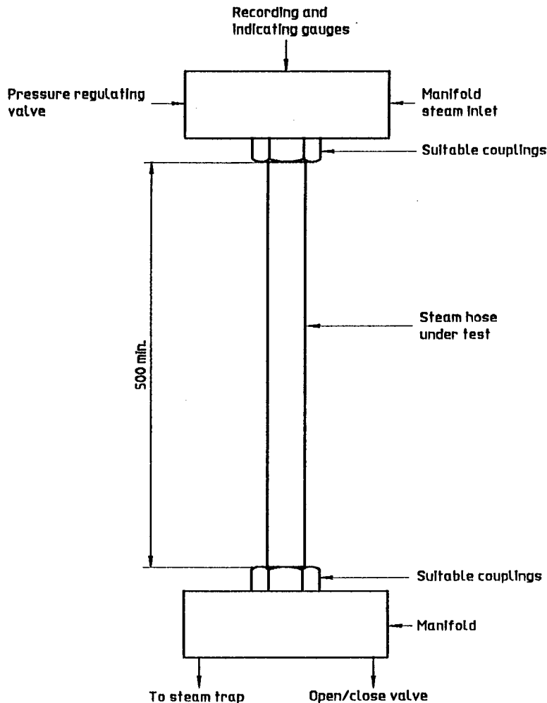
Figure 1 — Schematic diagram of arrangement for vertical steam rack test (method A)
