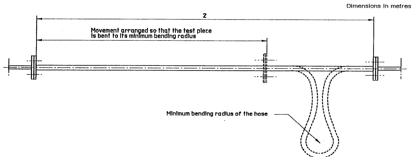
Figure 4 — Schematic diagram of arrangement for horizontal flexing test (method D)
