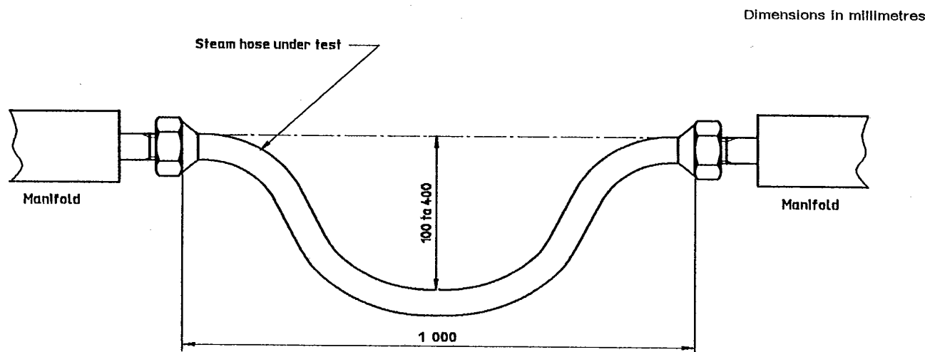
Figure 2 — Schematic diagram of arrangement for horizontal steam rack test (method B)
