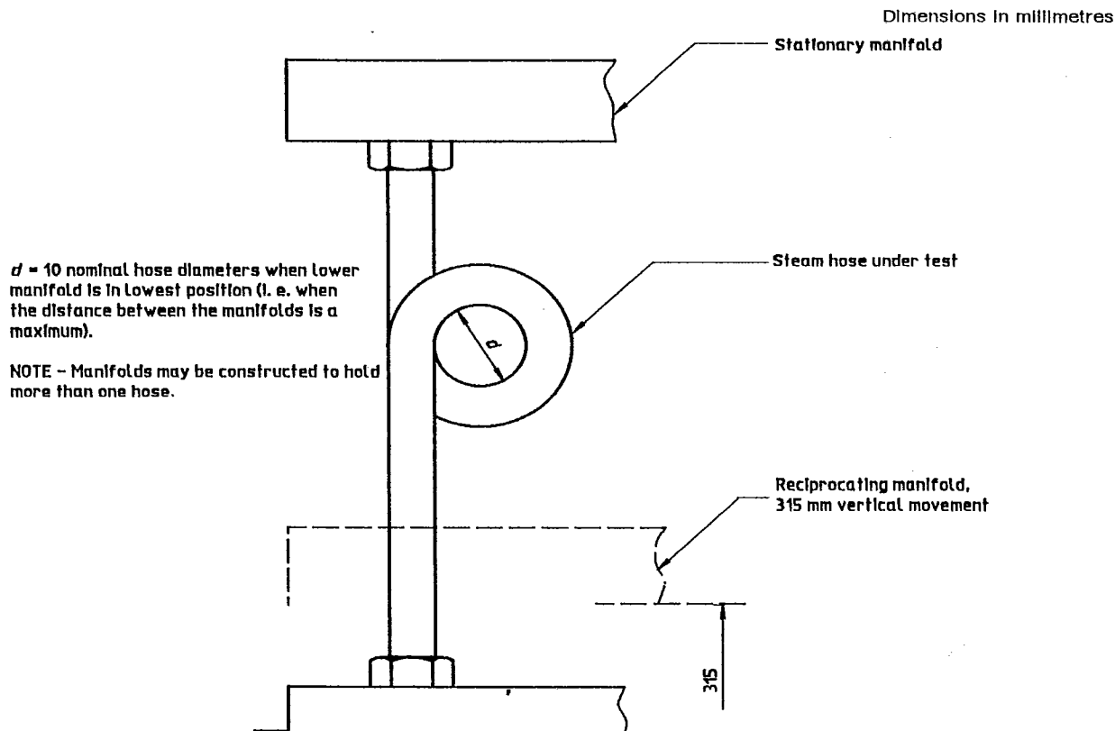
Figure 3 — Schematic diagram of arrangement for vertical flexing test (method C)
