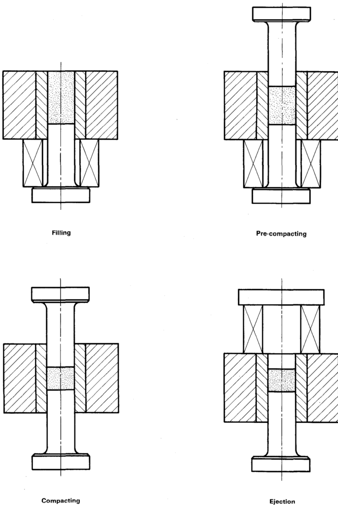
Figure 4 — Procedure of compacting and ejection
