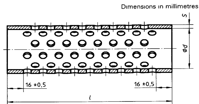
Figure 1 — Cylindrical tube
