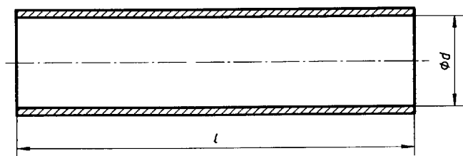
Figure 1 — Cylindrical tube
