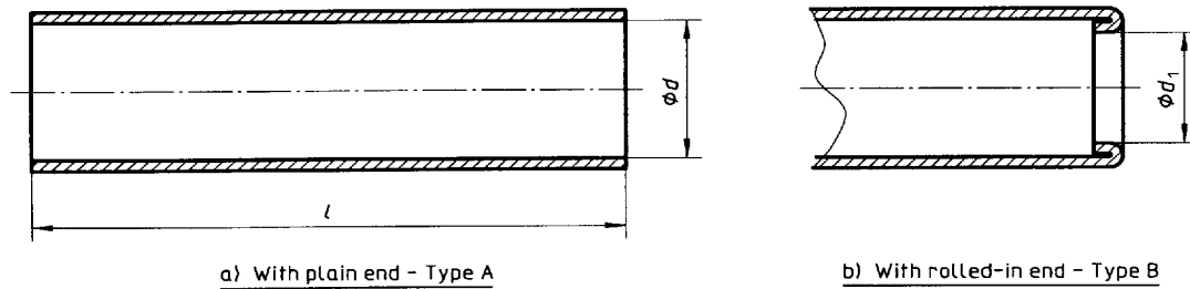
Figure 1 — Cylindrical tubes
