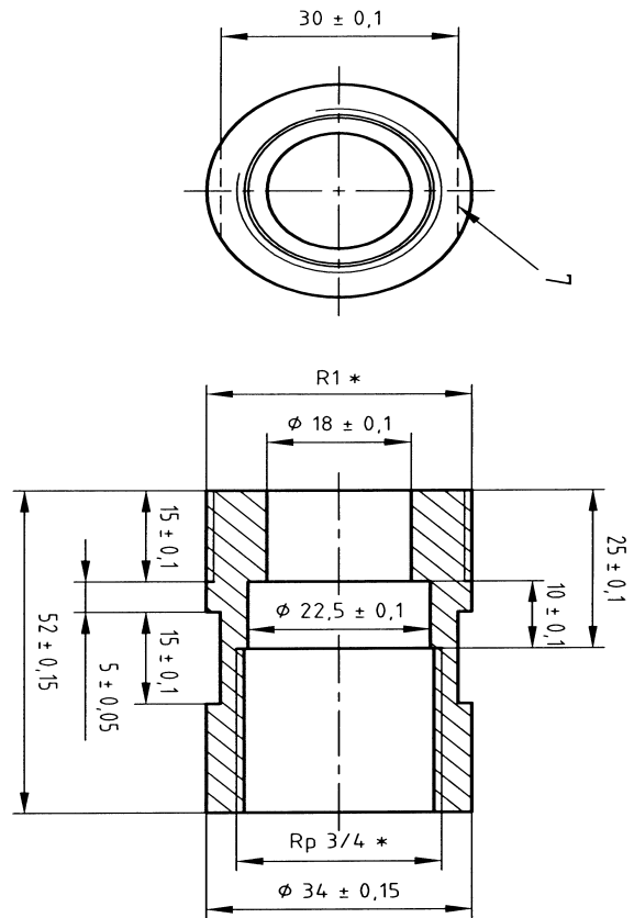
Figure 4d) - Receptacles
