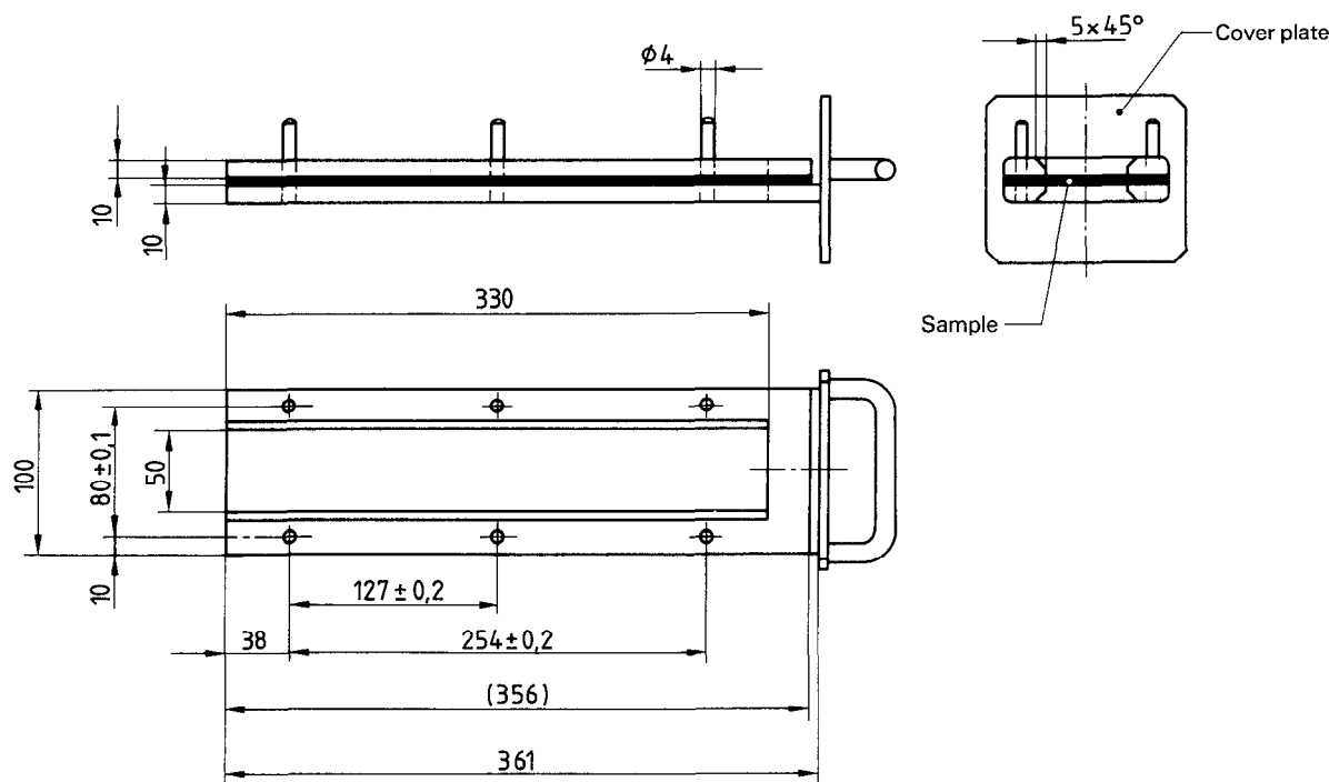
Figure 4 – Example of sample holder
