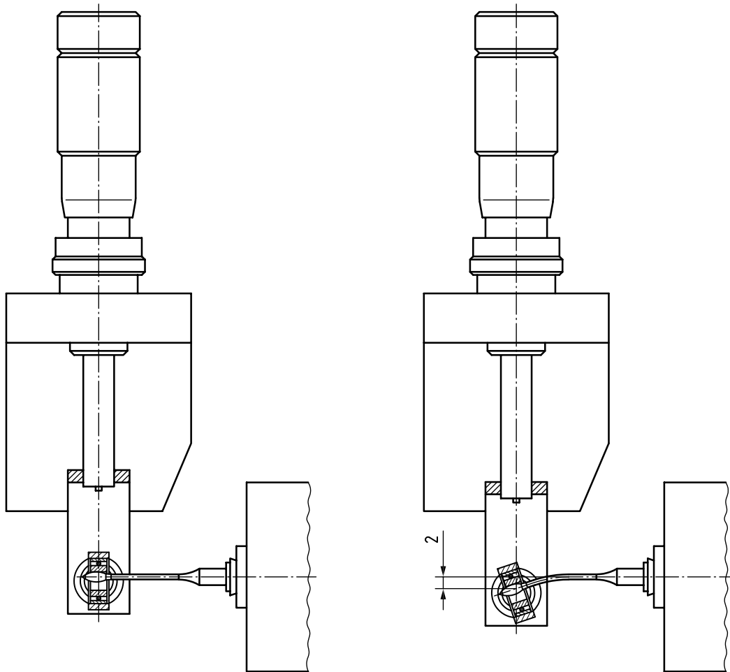
Figure 8 — Apparatus for testing resistance to fatigue
