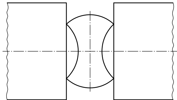
Figure 6 — Chucking position of instrument for testing twisting and angular deflection
