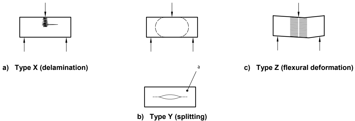
Figure 2 — Acceptable and unacceptable failure modes (Only Type X is acceptable)
