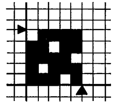
FIGURE 4b — Satin weave (warp faced)
