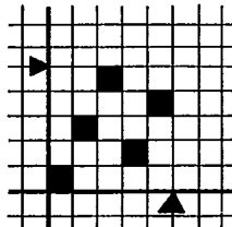
FIGURE 4a — Sateen weave (weft faced)
