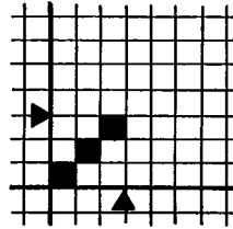
FIGURE 2a — Weft-faced "Z" twill weave
