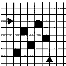
FIGURE 5a — Sateen weave (weft faced)
