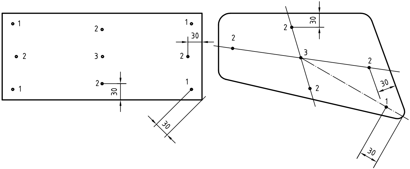
a) Flat or cylindrically curved safety glazing materials
