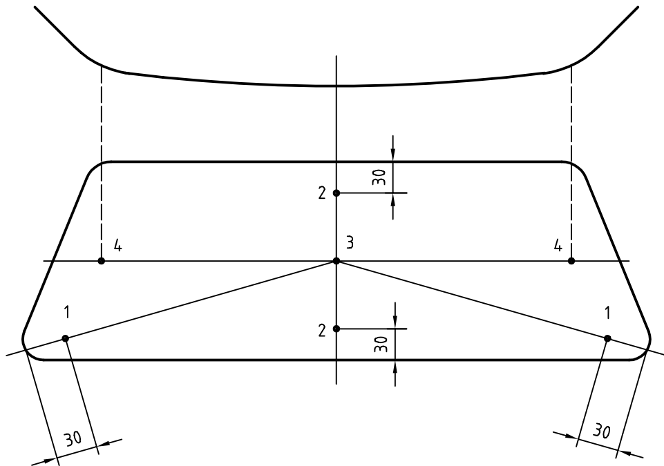
b) Complex-curved safety glazing materials
