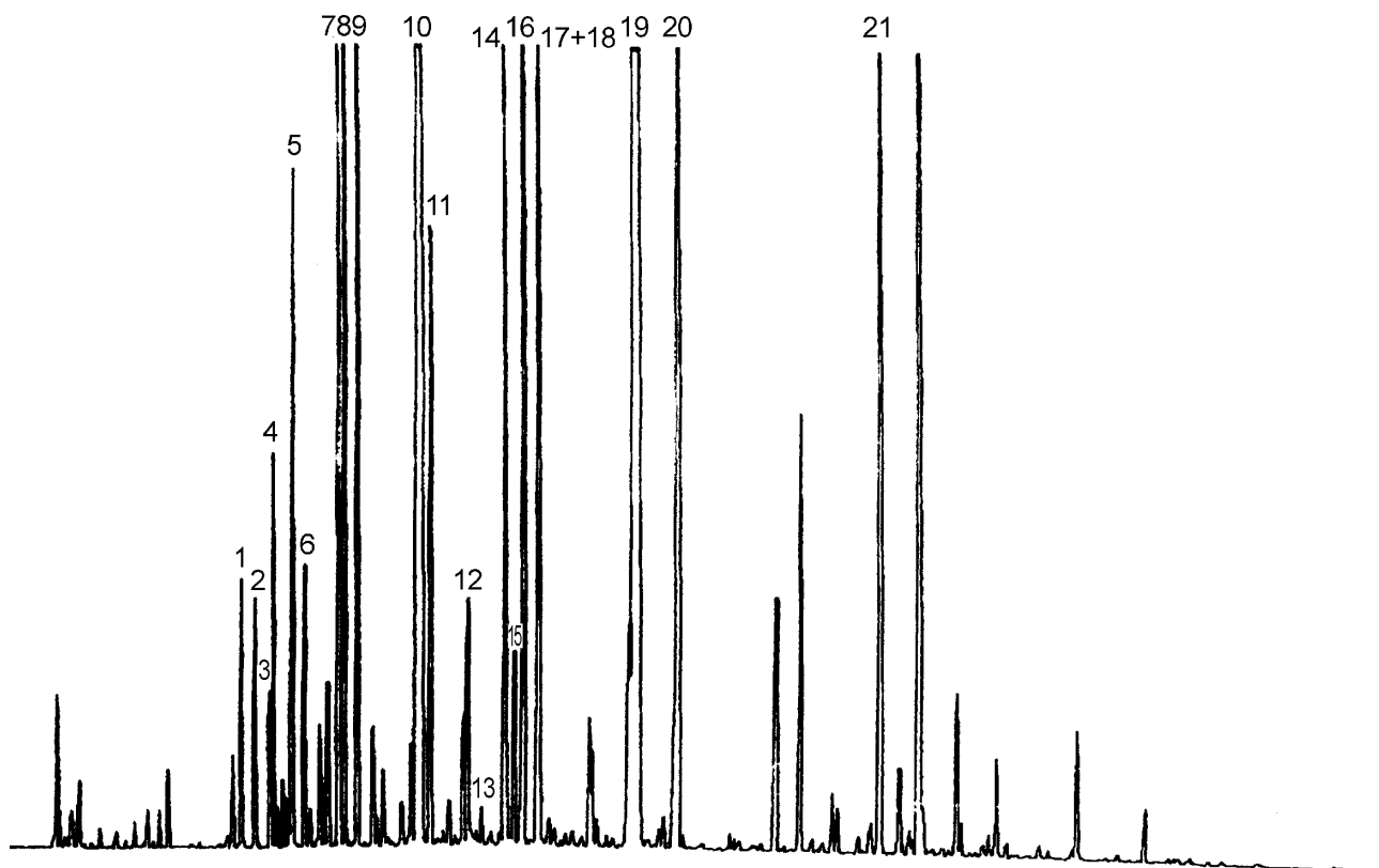
Figure B.3 — Typical chromatogram of clonal lavender, Bulgaria, taken on an apolar column
