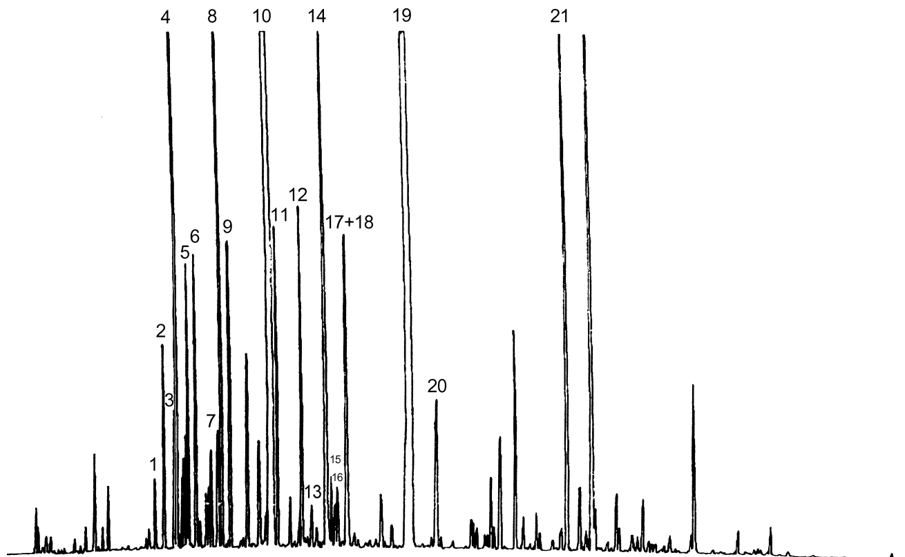
Figure B.1 — Typical chromatogram of clonal lavender, France "Maillette", taken on an apolar column
