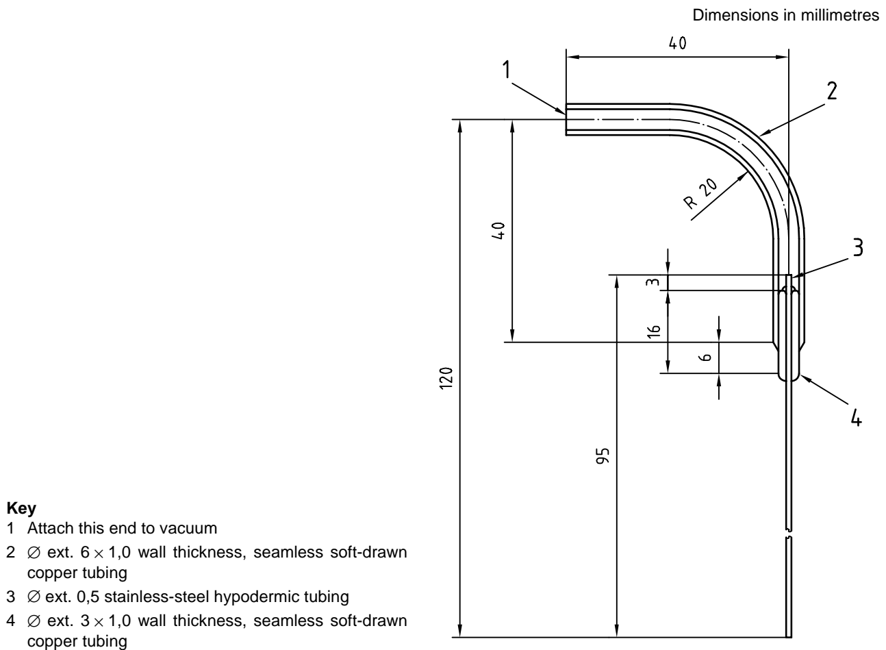
Figure A.1 — Draw-off needle
