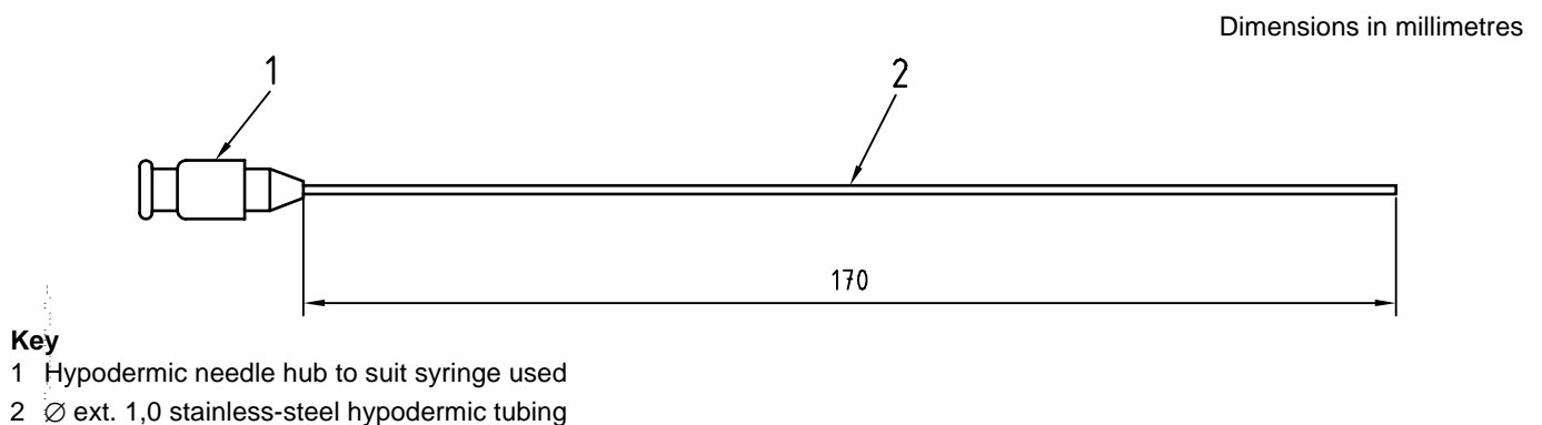
Figure A.2 — Filling needle
