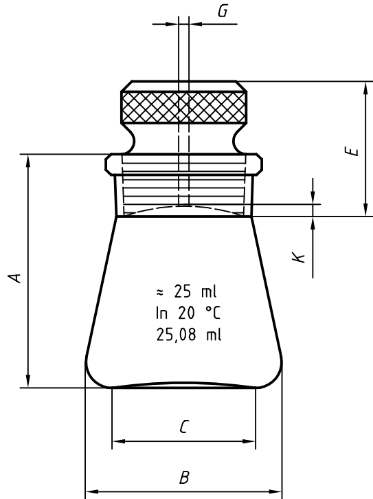
Figure 5 — Type 5 (Hubbard) pycnometer flask
