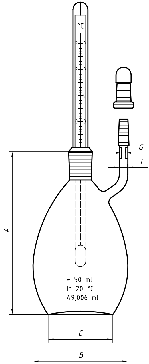
Figure 6 — Pycnometer flask with ground-in thermometer and capillary side tube
