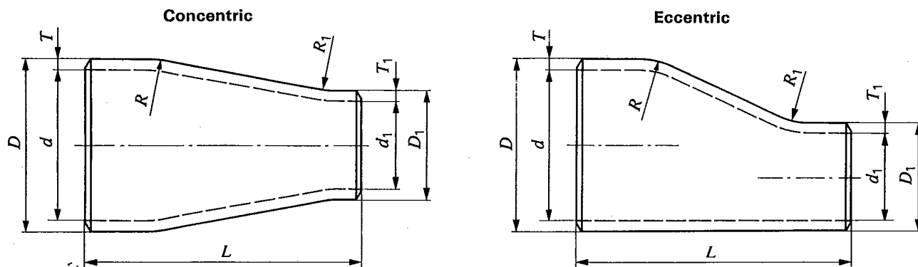
Figure 3 — Concentric and eccentric reducers
