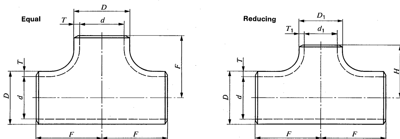
Figure 4 — Tees, equal and reducing
