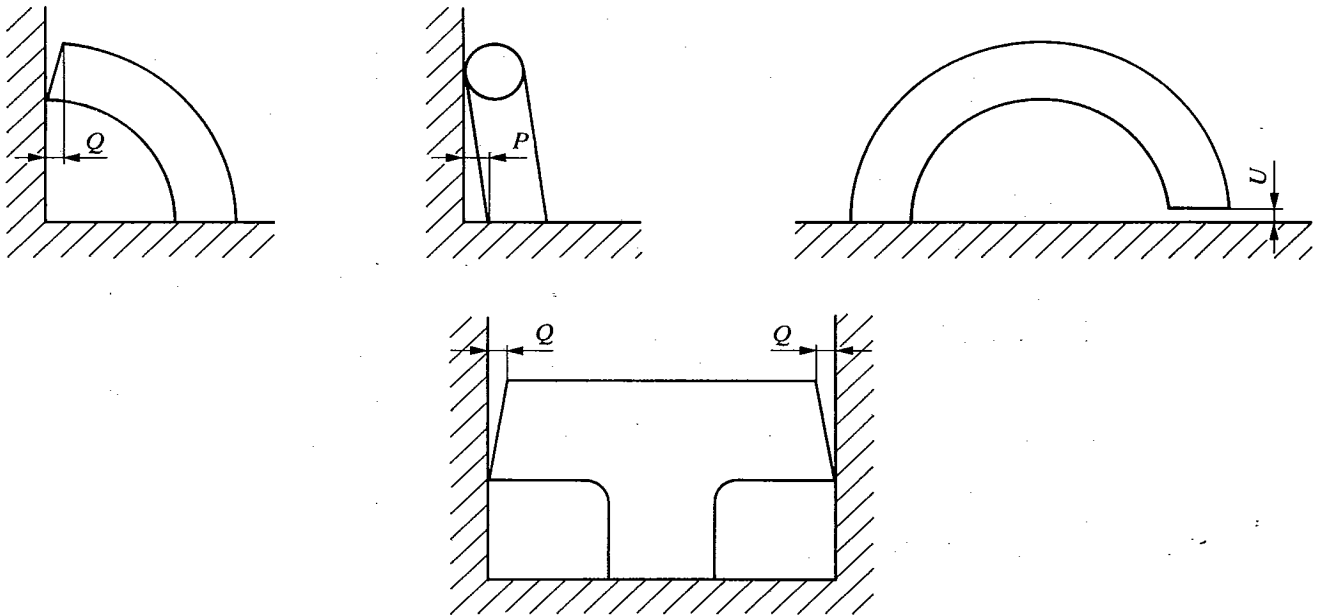
Figure 7 — Tolerances on alignment
