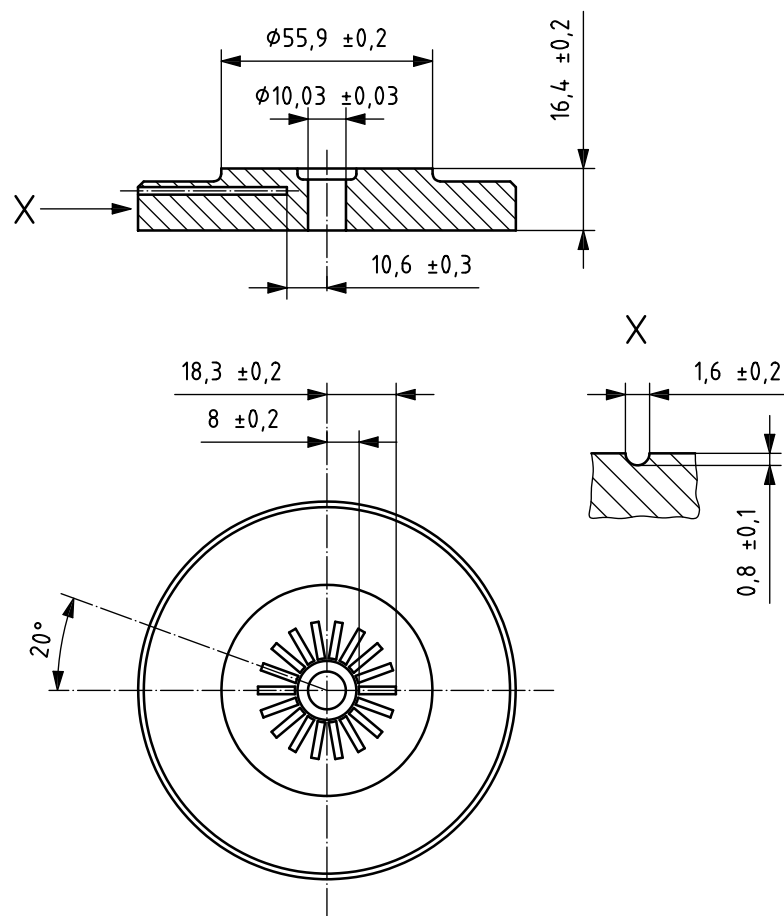
Figure 3 — Lower die
