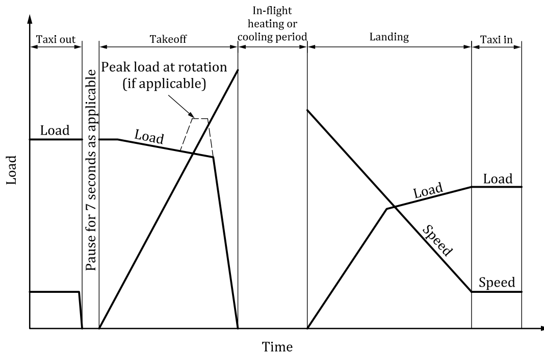
Figure 6 — Test cycle sequence — Total sortie
