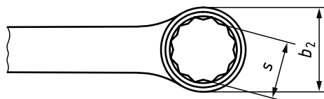
Figure 2 — Box end
