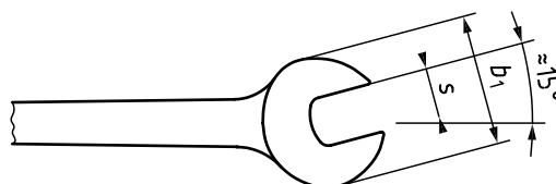
Figure 1 — Open-end
