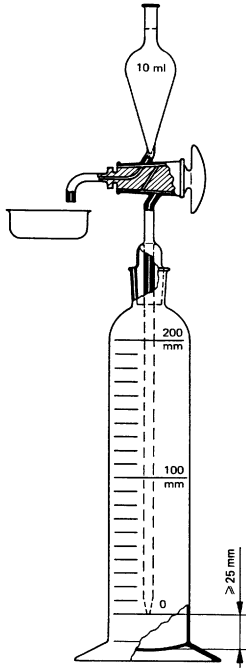
FIGURE 1 - Sedimentation vessel and pipette
