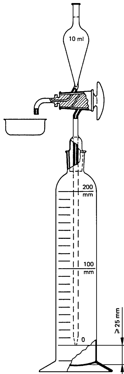
Figure 1 — Sedimentation vessel and pipette
