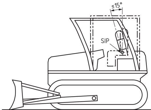
b) Longitudinal load on tractor-dozer
