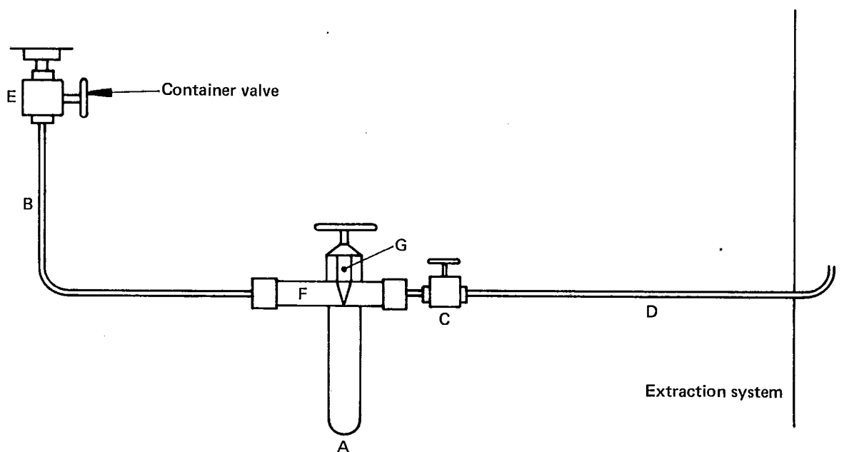
FIGURE 1 — Apparatus for sampling anhydrous hydrogen fluoride
