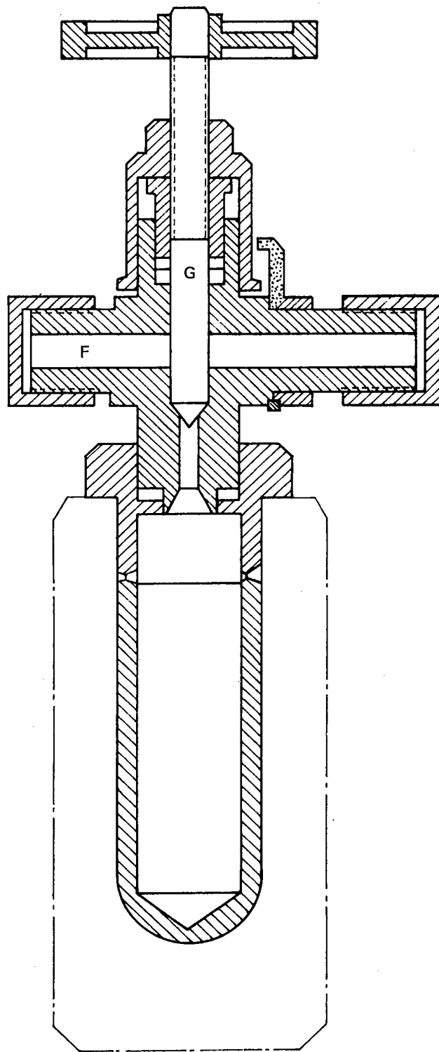
FIGURE 2 — Sample cylinder for anhydrous hydrogen fluoride (simplified diagram)
