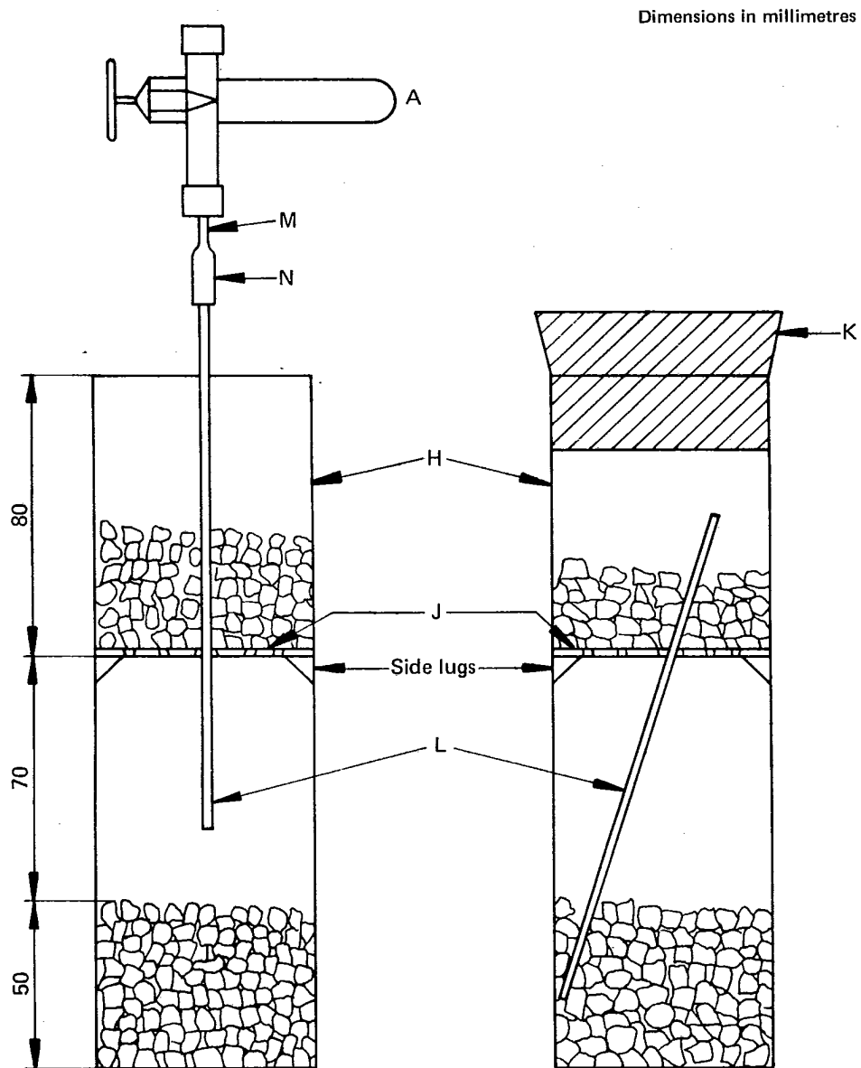
FIGURE 3 — Apparatus for preparing test samples of anhydrous hydrogen fluoride
