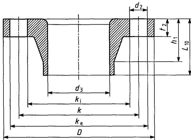
Figure 6 — Flange dimensions
